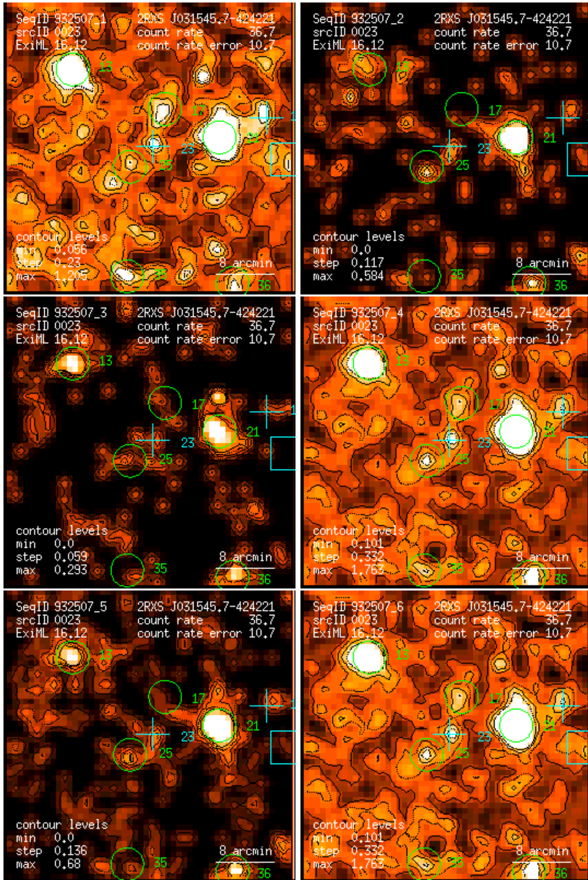
Figure 23: RASS 932507: detection 0023: band rate images, Gaussian filter: (1) PSPC channels 11 – 41, (2) 52 – 90, (3) 91 – 201, (4) 11 – 235, (5) 52 – 201, (6) 11 – 201. Broad band rates in counts/ks. Band rate contour levels in counts/ks/arcmin 2 .
