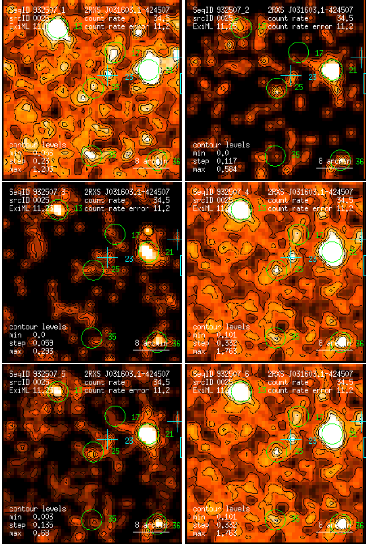
Figure 25: RASS 932507: detection 0025: band rate images, Gaussian filter: (1) PSPC channels 11 – 41, (2) 52 – 90, (3) 91 – 201, (4) 11 – 235, (5) 52 – 201, (6) 11 – 201. Broad band rates in counts/ks. Band rate contour levels in counts/ks/arcmin 2 .
