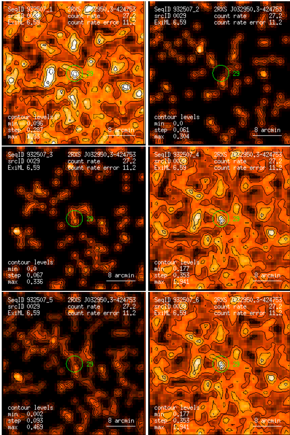
Figure 29: RASS 932507: detection 0029: band rate images, Gaussian filter: (1) PSPC channels 11 – 41, (2) 52 – 90, (3) 91 – 201, (4) 11 – 235, (5) 52 – 201, (6) 11 – 201. Broad band rates in counts/ks. Band rate contour levels in counts/ks/arcmin 2 .
