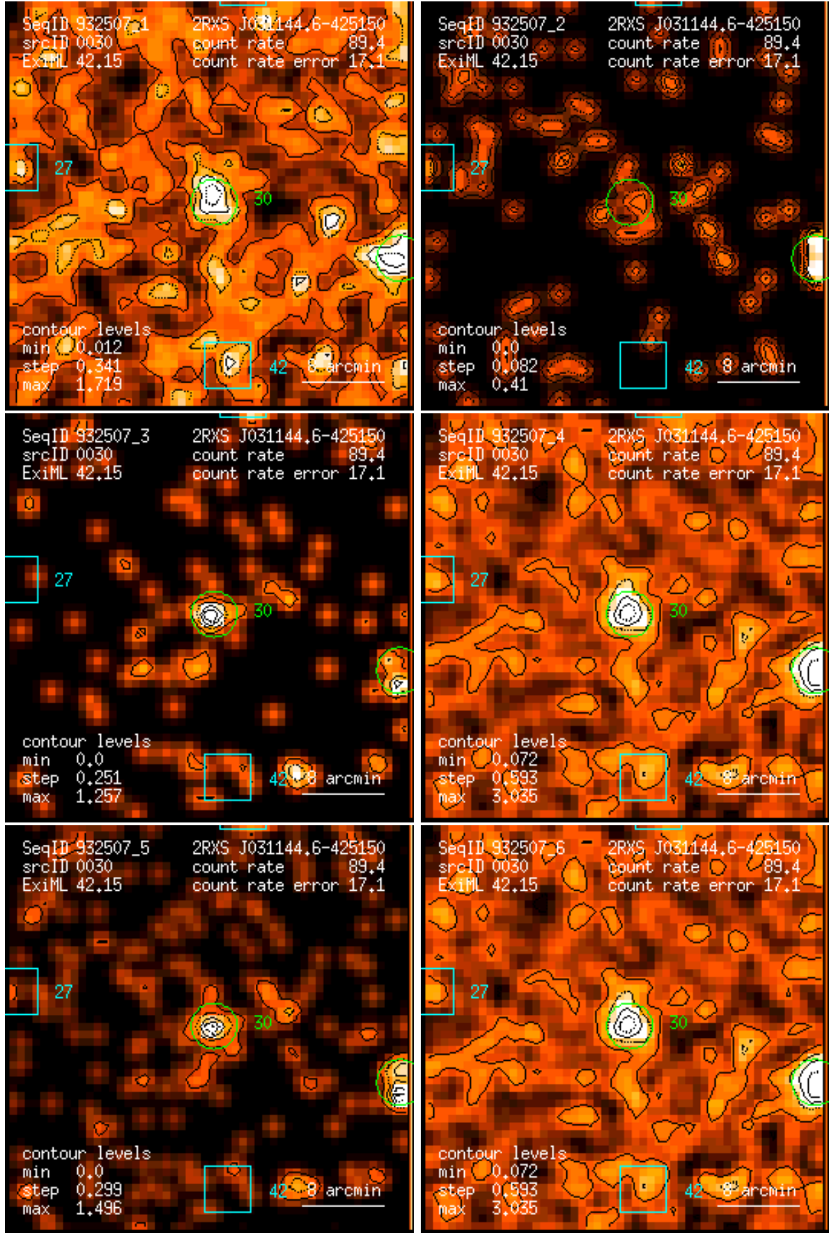
Figure 30: RASS 932507: detection 0030: band rate images, Gaussian filter: (1) PSPC channels 11 – 41, (2) 52 – 90, (3) 91 – 201, (4) 11 – 235, (5) 52 – 201, (6) 11 – 201. Broad band rates in counts/ks. Band rate contour levels in counts/ks/arcmin 2 .
