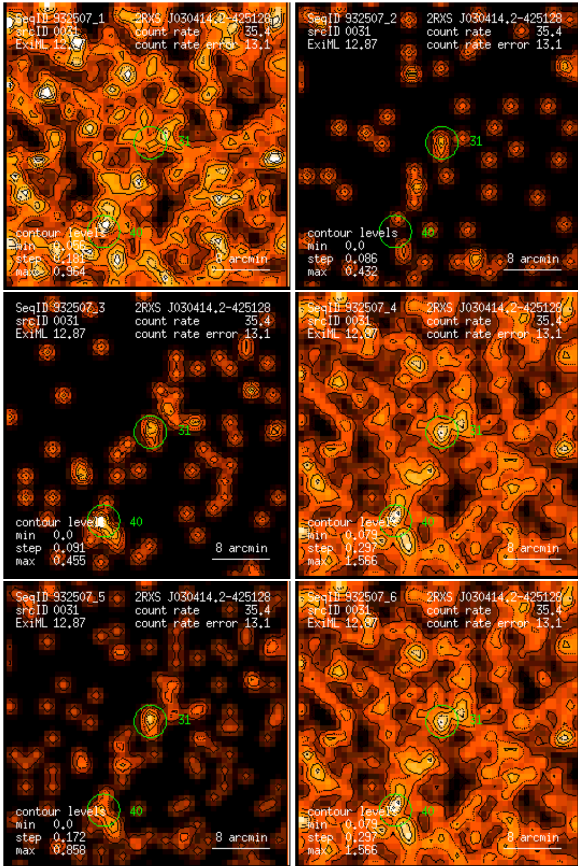
Figure 31: RASS 932507: detection 0031: band rate images, Gaussian filter: (1) PSPC channels 11 – 41, (2) 52 – 90, (3) 91 – 201, (4) 11 – 235, (5) 52 – 201, (6) 11 – 201. Broad band rates in counts/ks. Band rate contour levels in counts/ks/arcmin 2 .
