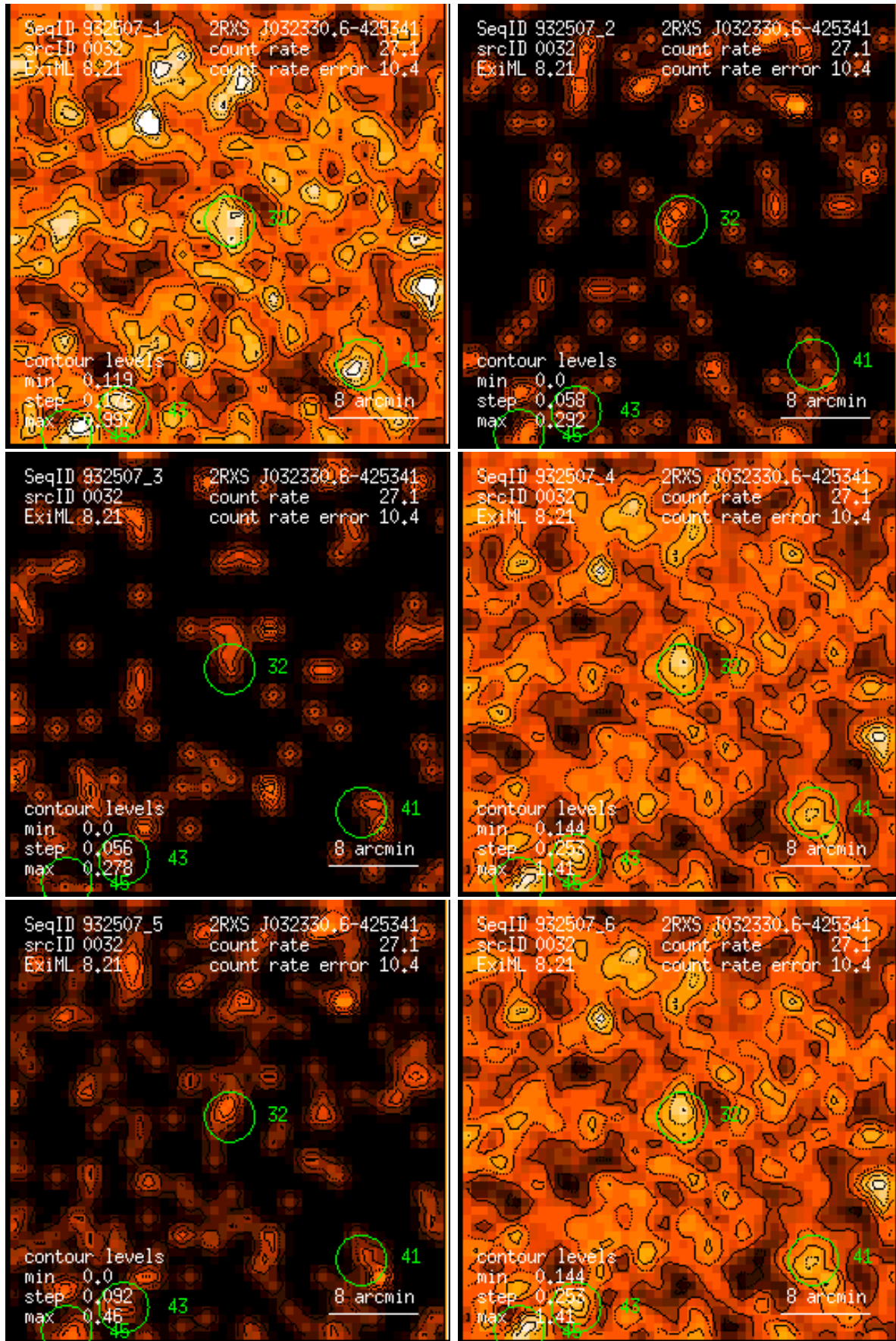
Figure 32: RASS 932507: detection 0032: band rate images, Gaussian filter: (1) PSPC channels 11 – 41, (2) 52 – 90, (3) 91 – 201, (4) 11 – 235, (5) 52 – 201, (6) 11 – 201. Broad band rates in counts/ks. Band rate contour levels in counts/ks/arcmin 2 .
