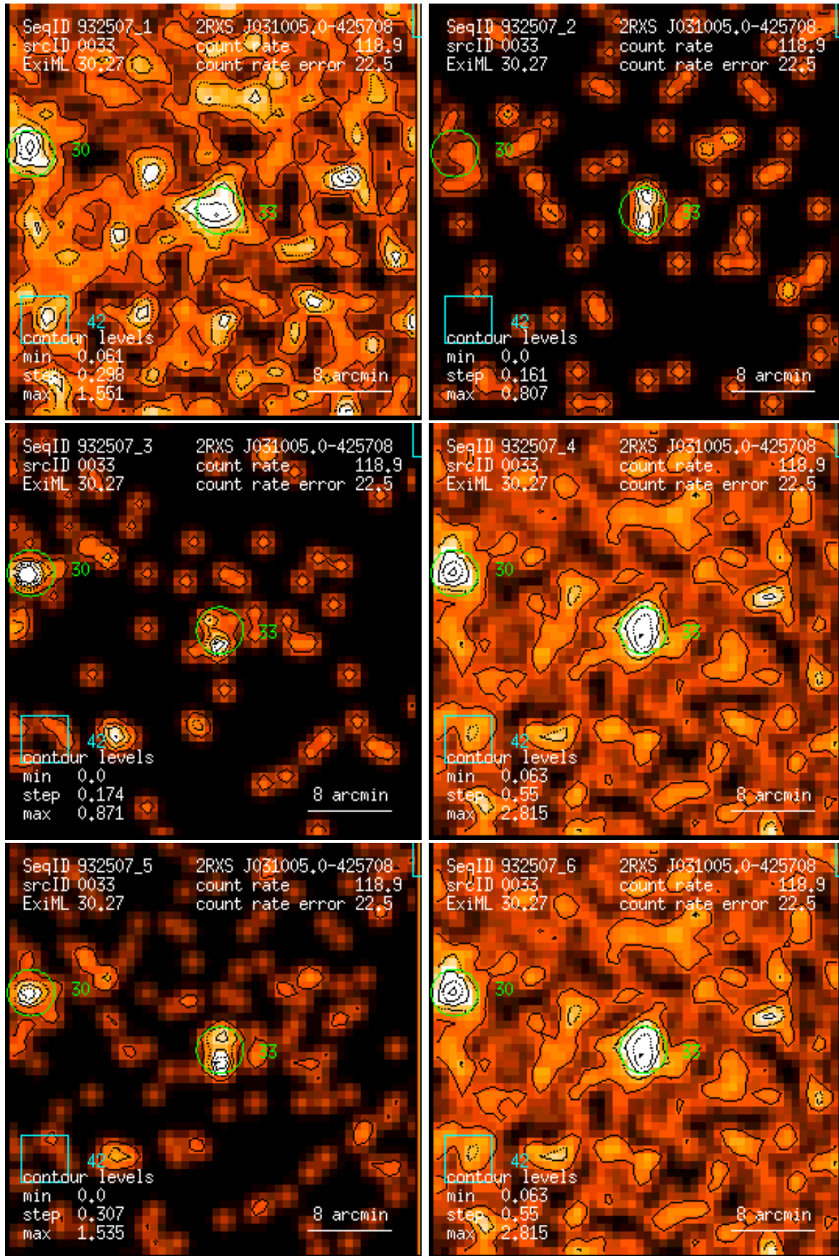
Figure 33: RASS 932507: detection 0033: band rate images, Gaussian filter: (1) PSPC channels 11 – 41, (2) 52 – 90, (3) 91 – 201, (4) 11 – 235, (5) 52 – 201, (6) 11 – 201. Broad band rates in counts/ks. Band rate contour levels in counts/ks/arcmin 2 .
