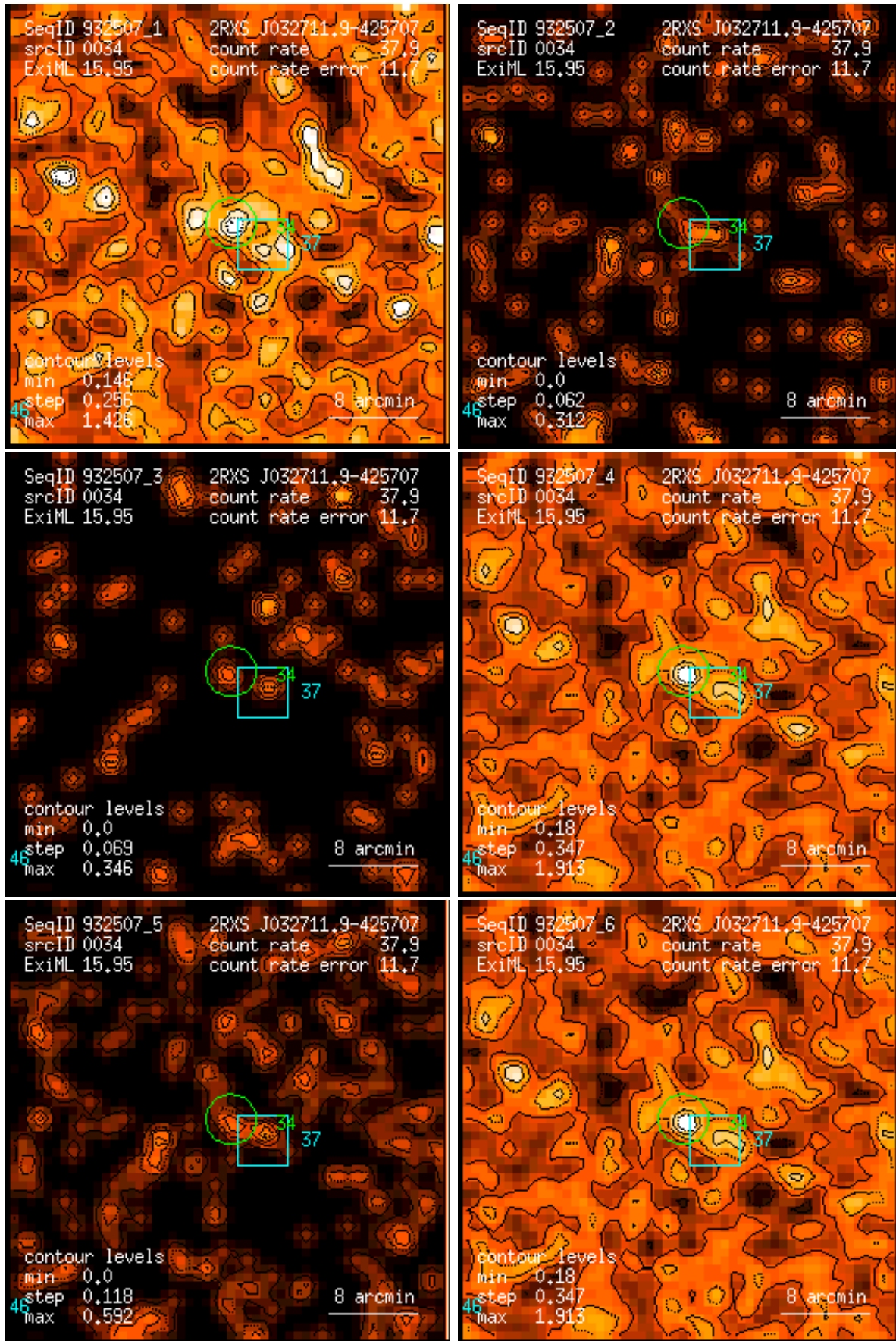
Figure 34: RASS 932507: detection 0034: band rate images, Gaussian filter: (1) PSPC channels 11 – 41, (2) 52 – 90, (3) 91 – 201, (4) 11 – 235, (5) 52 – 201, (6) 11 – 201. Broad band rates in counts/ks. Band rate contour levels in counts/ks/arcmin 2 .
