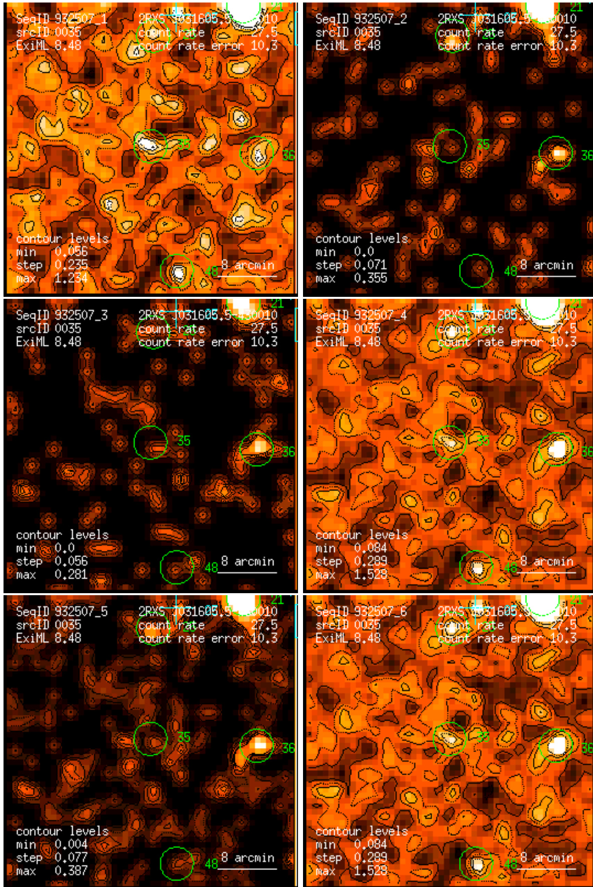
Figure 35: RASS 932507: detection 0035: band rate images, Gaussian filter: (1) PSPC channels 11 – 41, (2) 52 – 90, (3) 91 – 201, (4) 11 – 235, (5) 52 – 201, (6) 11 – 201. Broad band rates in counts/ks. Band rate contour levels in counts/ks/arcmin 2 .
