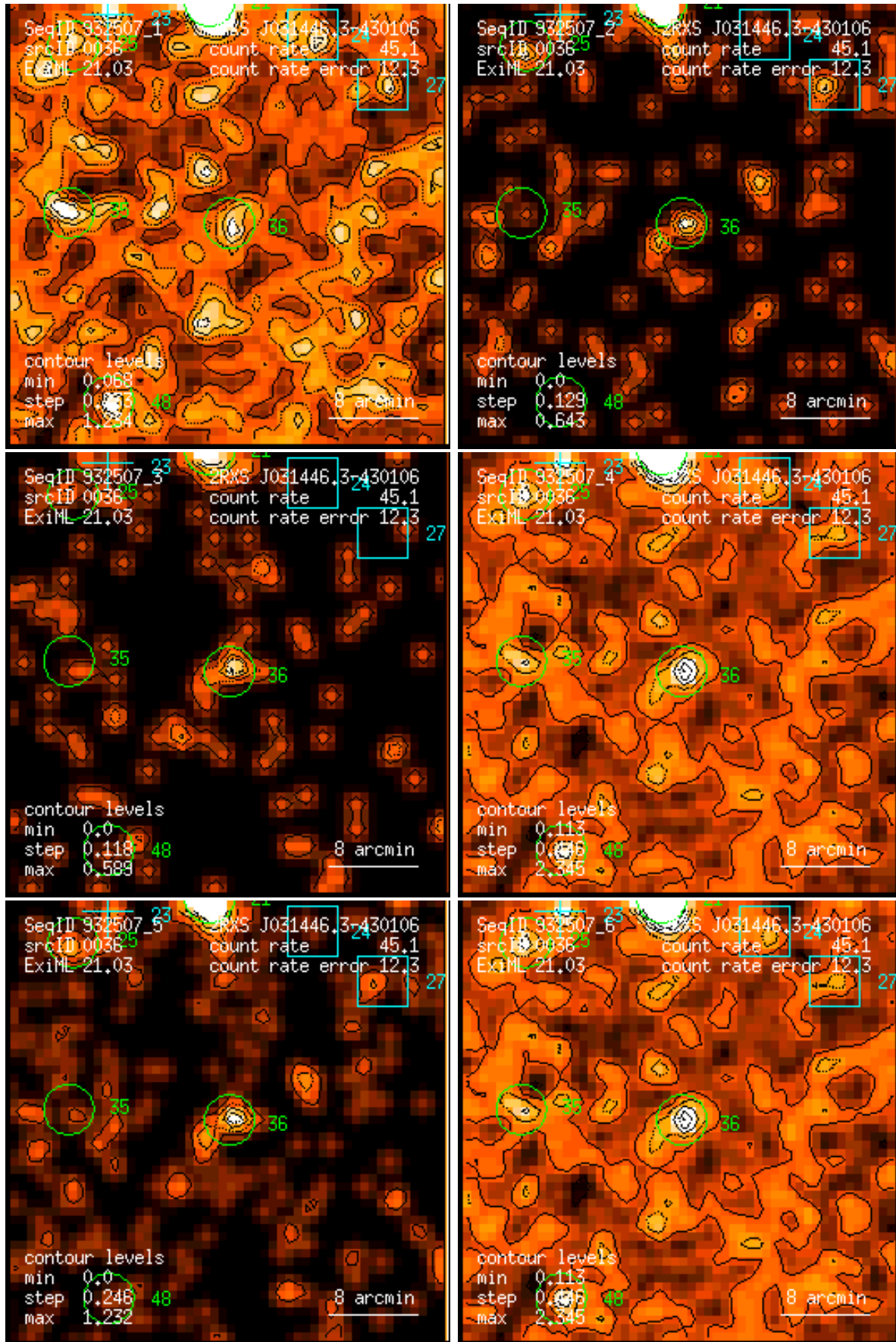
Figure 36: RASS 932507: detection 0036: band rate images, Gaussian filter: (1) PSPC channels 11 – 41, (2) 52 – 90, (3) 91 – 201, (4) 11 – 235, (5) 52 – 201, (6) 11 – 201. Broad band rates in counts/ks. Band rate contour levels in counts/ks/arcmin 2 .
