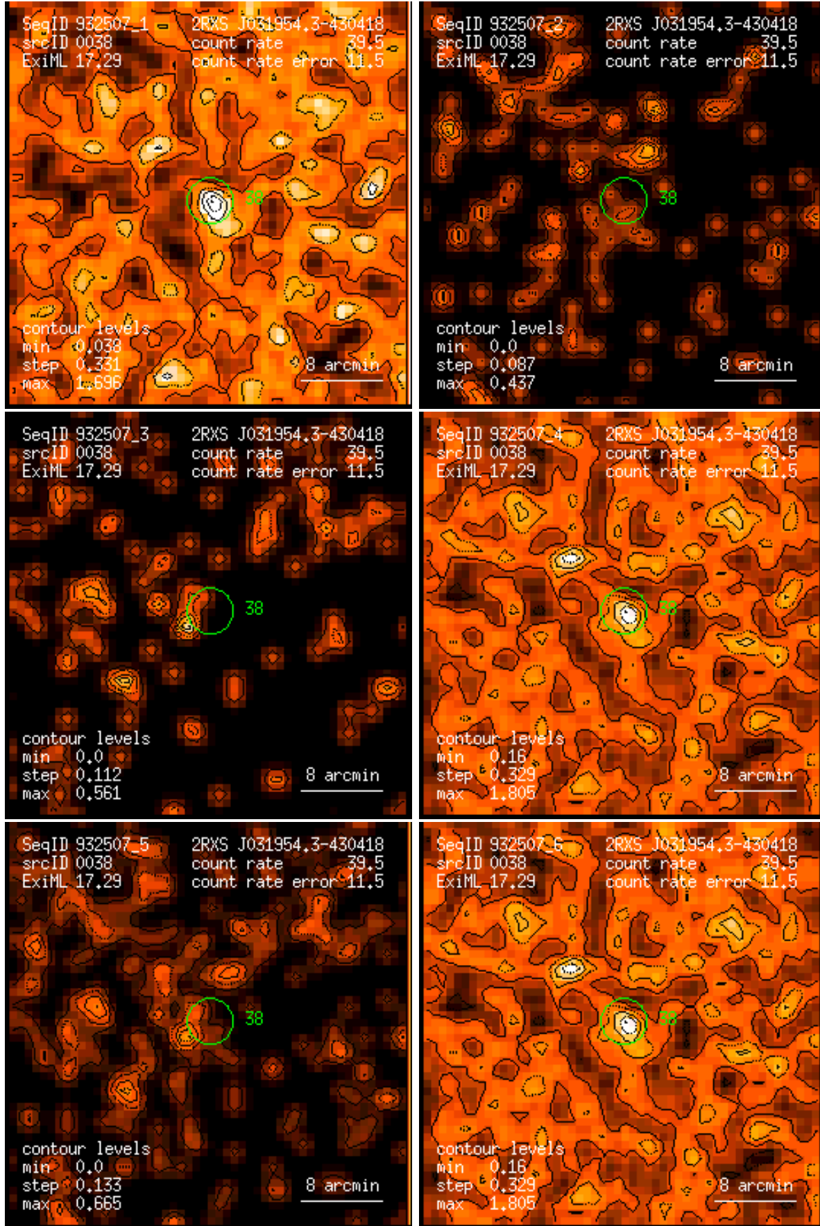
Figure 38: RASS 932507: detection 0038: band rate images, Gaussian filter: (1) PSPC channels 11 – 41, (2) 52 – 90, (3) 91 – 201, (4) 11 – 235, (5) 52 – 201, (6) 11 – 201. Broad band rates in counts/ks. Band rate contour levels in counts/ks/arcmin 2 .
