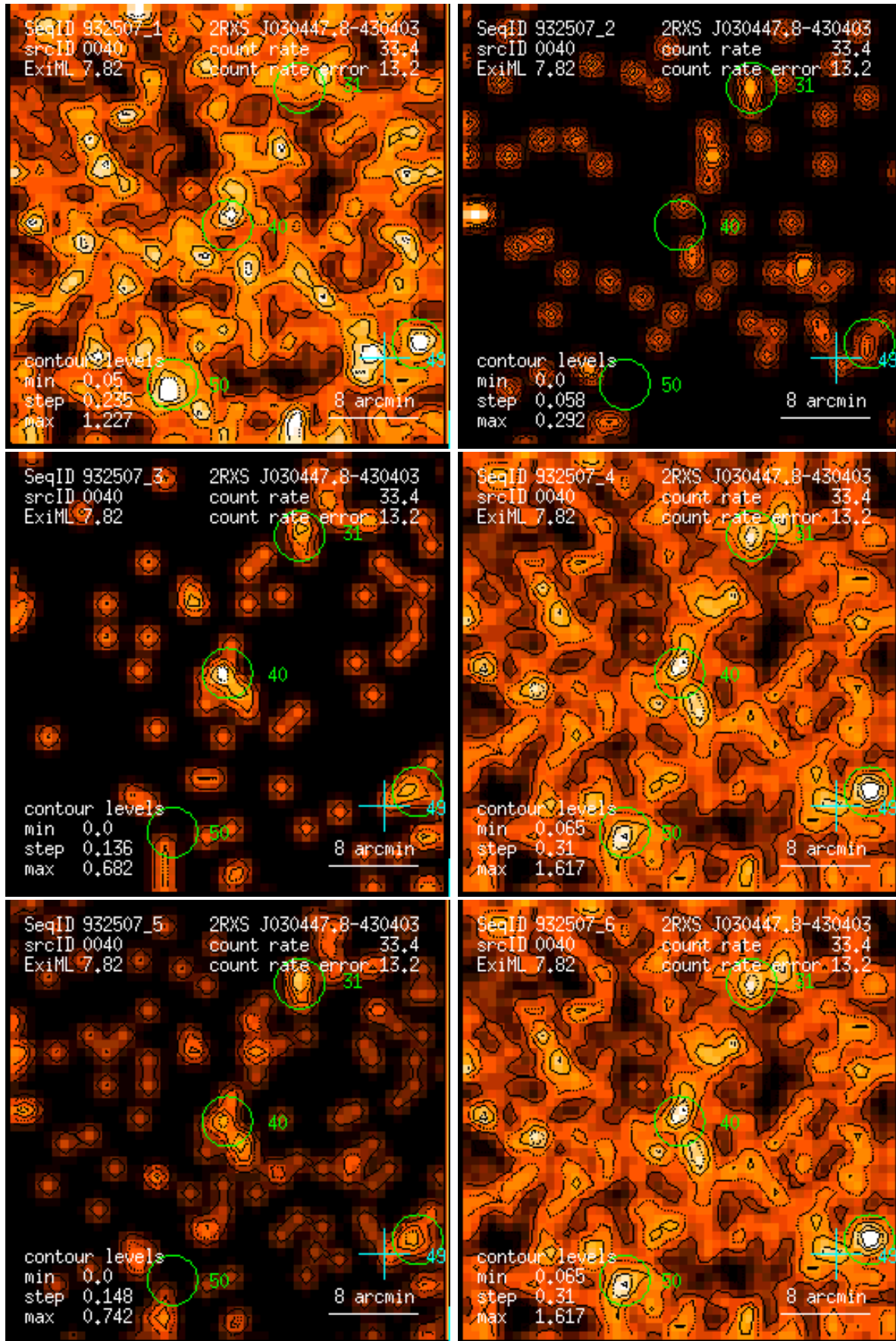
Figure 40: RASS 932507: detection 0040: band rate images, Gaussian filter: (1) PSPC channels 11 – 41, (2) 52 – 90, (3) 91 – 201, (4) 11 – 235, (5) 52 – 201, (6) 11 – 201. Broad band rates in counts/ks. Band rate contour levels in counts/ks/arcmin 2 .
