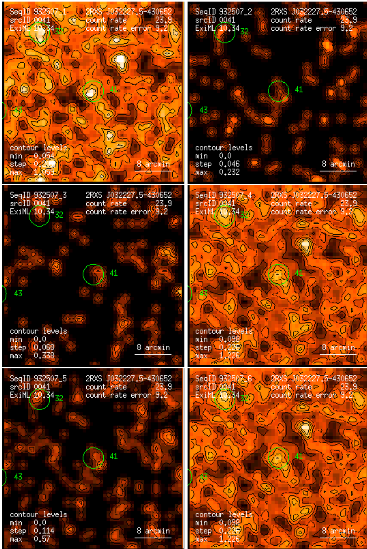
Figure 41: RASS 932507: detection 0041: band rate images, Gaussian filter: (1) PSPC channels 11 – 41, (2) 52 – 90, (3) 91 – 201, (4) 11 – 235, (5) 52 – 201, (6) 11 – 201. Broad band rates in counts/ks. Band rate contour levels in counts/ks/arcmin 2 .
