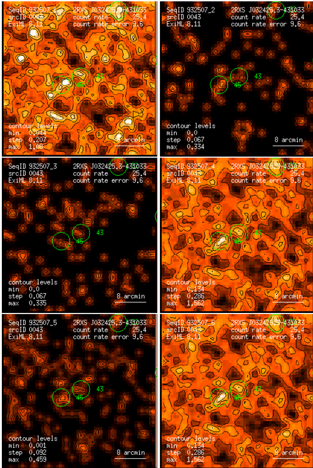
Figure 43: RASS 932507: detection 0043: band rate images, Gaussian filter: (1) PSPC channels 11 – 41, (2) 52 – 90, (3) 91 – 201, (4) 11 – 235, (5) 52 – 201, (6) 11 – 201. Broad band rates in counts/ks. Band rate contour levels in counts/ks/arcmin 2 .
