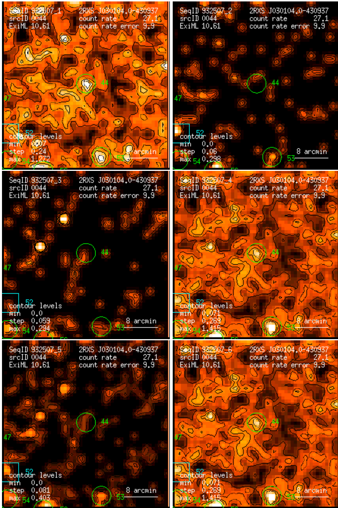
Figure 44: RASS 932507: detection 0044: band rate images, Gaussian filter: (1) PSPC channels 11 – 41, (2) 52 – 90, (3) 91 – 201, (4) 11 – 235, (5) 52 – 201, (6) 11 – 201. Broad band rates in counts/ks. Band rate contour levels in counts/ks/arcmin 2 .
