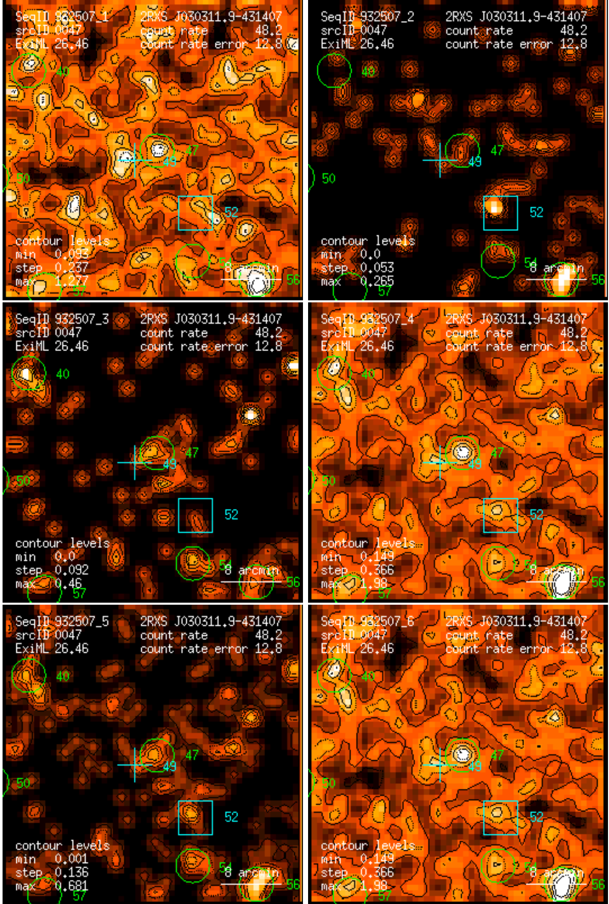
Figure 47: RASS 932507: detection 0047: band rate images, Gaussian filter: (1) PSPC channels 11 – 41, (2) 52 – 90, (3) 91 – 201, (4) 11 – 235, (5) 52 – 201, (6) 11 – 201. Broad band rates in counts/ks. Band rate contour levels in counts/ks/arcmin 2 .
