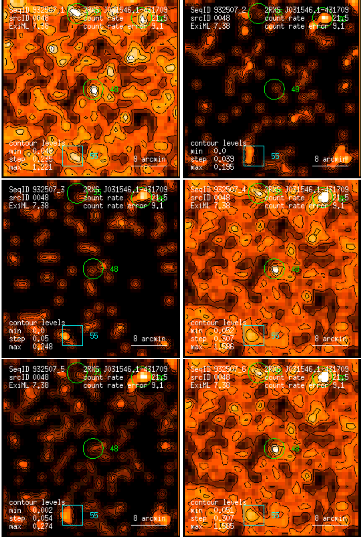
Figure 48: RASS 932507: detection 0048: band rate images, Gaussian filter: (1) PSPC channels 11 – 41, (2) 52 – 90, (3) 91 – 201, (4) 11 – 235, (5) 52 – 201, (6) 11 – 201. Broad band rates in counts/ks. Band rate contour levels in counts/ks/arcmin 2 .
