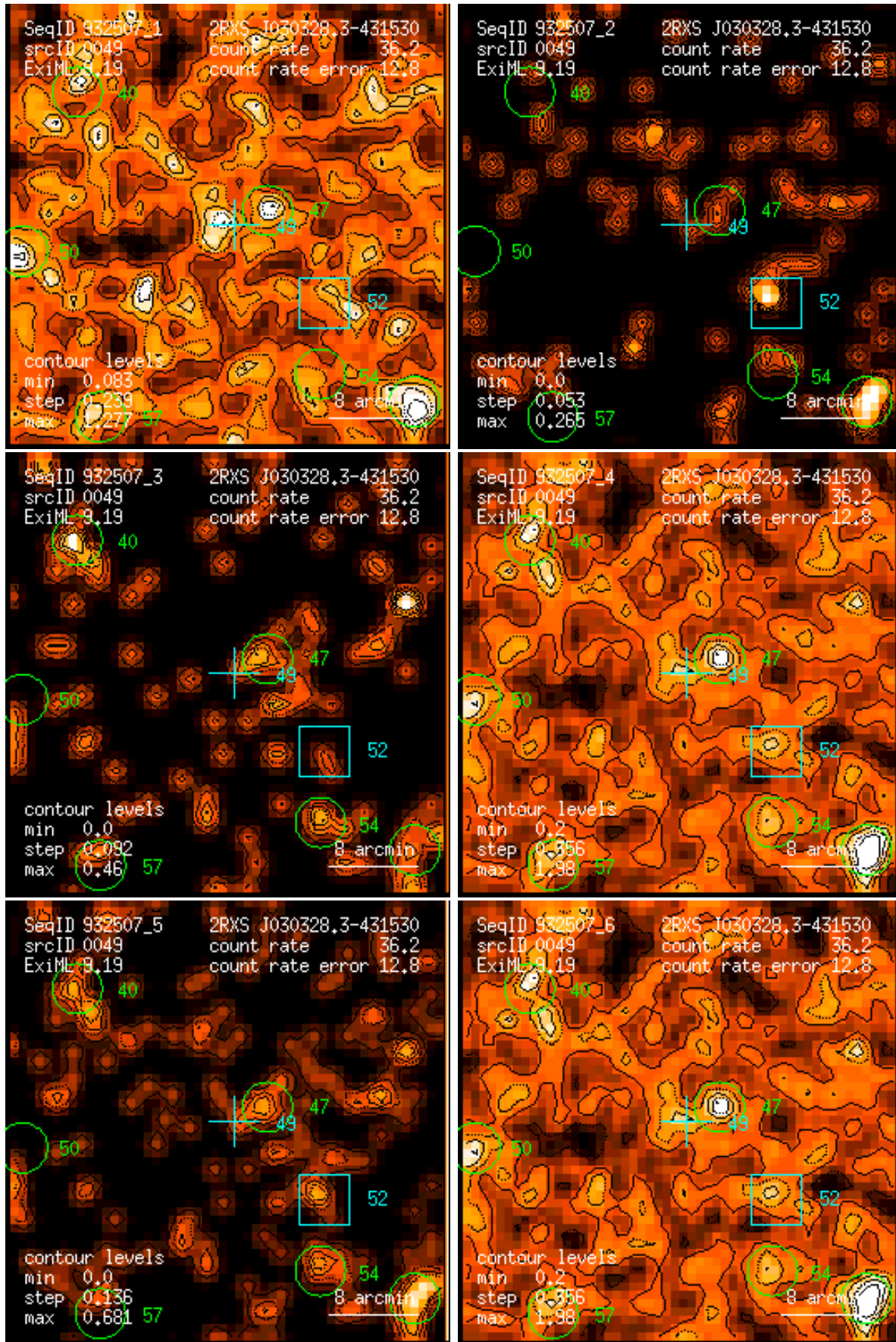
Figure 49: RASS 932507: detection 0049: band rate images, Gaussian filter: (1) PSPC channels 11 – 41, (2) 52 – 90, (3) 91 – 201, (4) 11 – 235, (5) 52 – 201, (6) 11 – 201. Broad band rates in counts/ks. Band rate contour levels in counts/ks/arcmin 2 .
