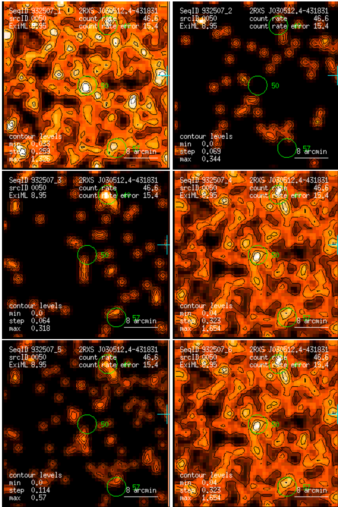
Figure 50: RASS 932507: detection 0050: band rate images, Gaussian filter: (1) PSPC channels 11 – 41, (2) 52 – 90, (3) 91 – 201, (4) 11 – 235, (5) 52 – 201, (6) 11 – 201. Broad band rates in counts/ks. Band rate contour levels in counts/ks/arcmin 2 .
