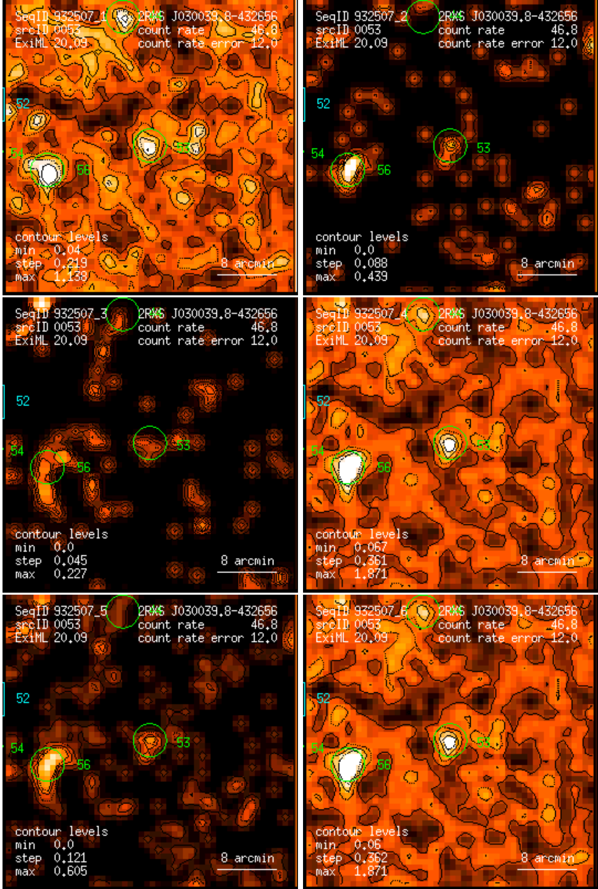
Figure 53: RASS 932507: detection 0053: band rate images, Gaussian filter: (1) PSPC channels 11 – 41, (2) 52 – 90, (3) 91 – 201, (4) 11 – 235, (5) 52 – 201, (6) 11 – 201. Broad band rates in counts/ks. Band rate contour levels in counts/ks/arcmin 2 .
