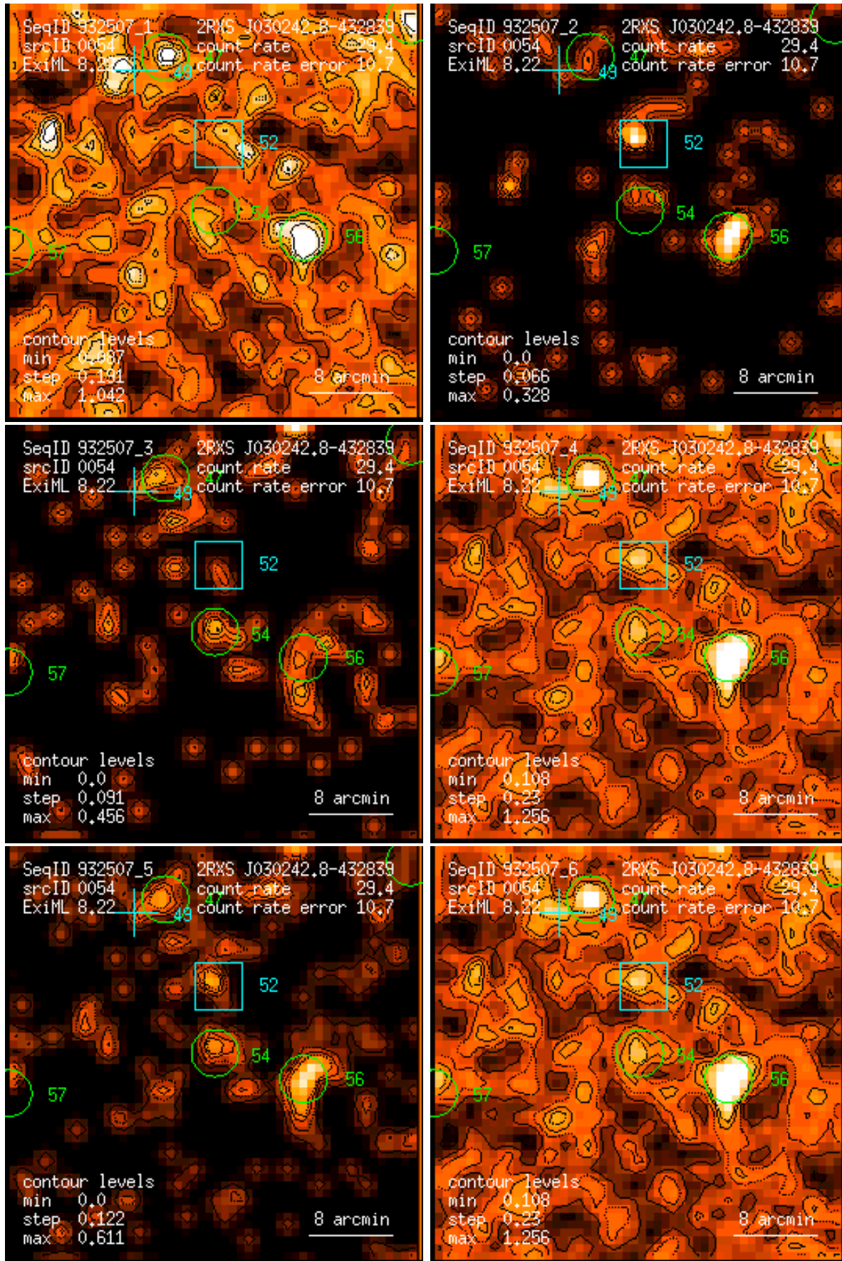
Figure 54: RASS 932507: detection 0054: band rate images, Gaussian filter: (1) PSPC channels 11 – 41, (2) 52 – 90, (3) 91 – 201, (4) 11 – 235, (5) 52 – 201, (6) 11 – 201. Broad band rates in counts/ks. Band rate contour levels in counts/ks/arcmin 2 .
