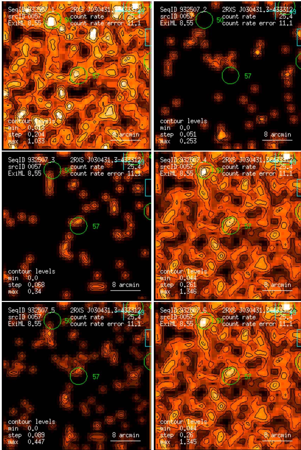
Figure 57: RASS 932507: detection 0057: band rate images, Gaussian filter: (1) PSPC channels 11 – 41, (2) 52 – 90, (3) 91 – 201, (4) 11 – 235, (5) 52 – 201, (6) 11 – 201. Broad band rates in counts/ks. Band rate contour levels in counts/ks/arcmin 2 .
