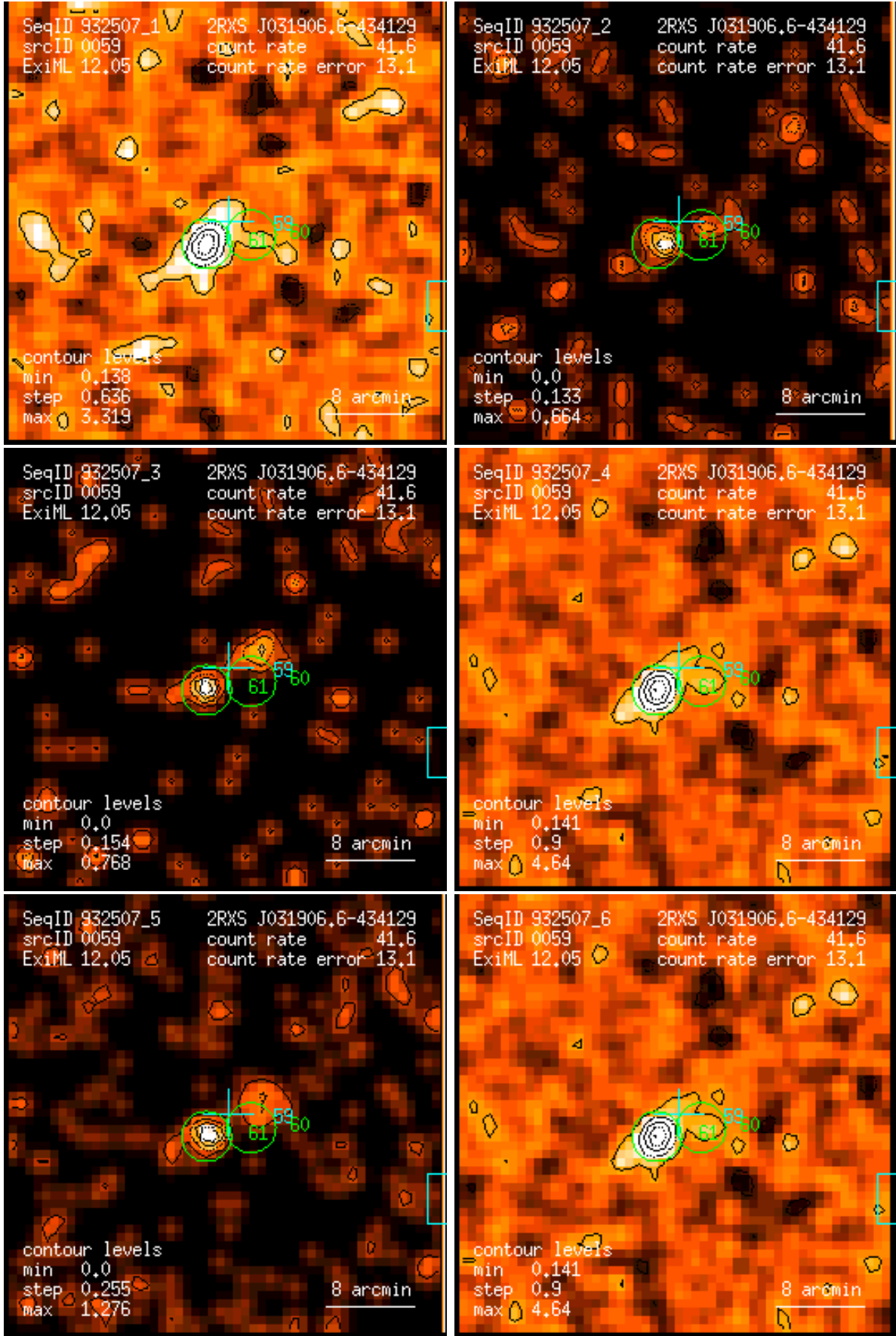
Figure 59: RASS 932507: detection 0059: band rate images, Gaussian filter: (1) PSPC channels 11 – 41, (2) 52 – 90, (3) 91 – 201, (4) 11 – 235, (5) 52 – 201, (6) 11 – 201. Broad band rates in counts/ks. Band rate contour levels in counts/ks/arcmin 2 .
