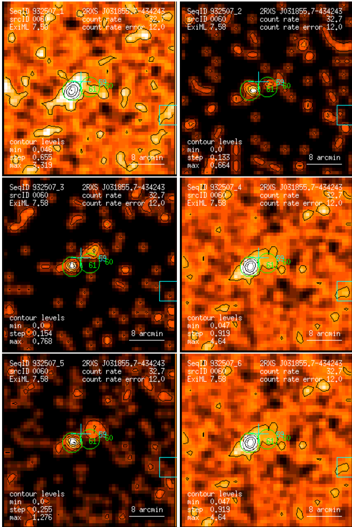
Figure 60: RASS 932507: detection 0060: band rate images, Gaussian filter: (1) PSPC channels 11 – 41, (2) 52 – 90, (3) 91 – 201, (4) 11 – 235, (5) 52 – 201, (6) 11 – 201. Broad band rates in counts/ks. Band rate contour levels in counts/ks/arcmin 2 .
