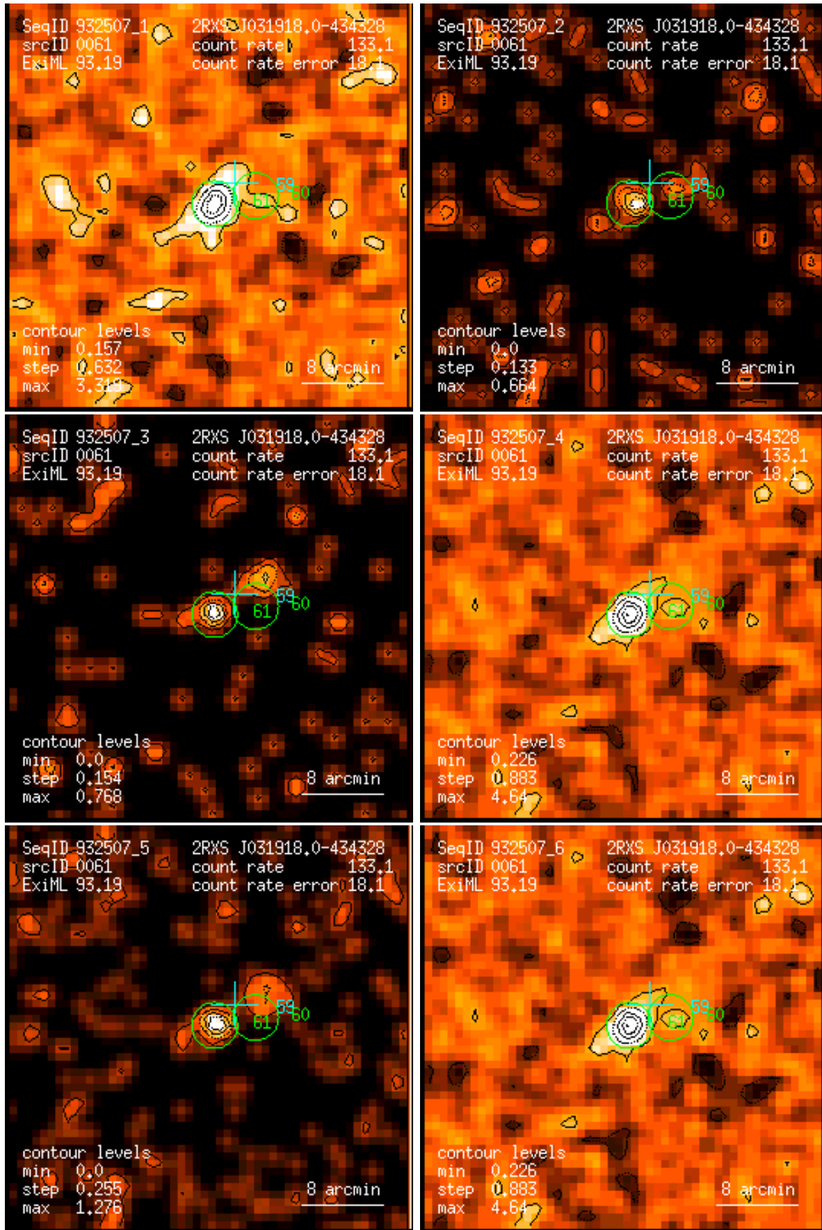
Figure 61: RASS 932507: detection 0061: band rate images, Gaussian filter: (1) PSPC channels 11 – 41, (2) 52 – 90, (3) 91 – 201, (4) 11 – 235, (5) 52 – 201, (6) 11 – 201. Broad band rates in counts/ks. Band rate contour levels in counts/ks/arcmin 2 .
