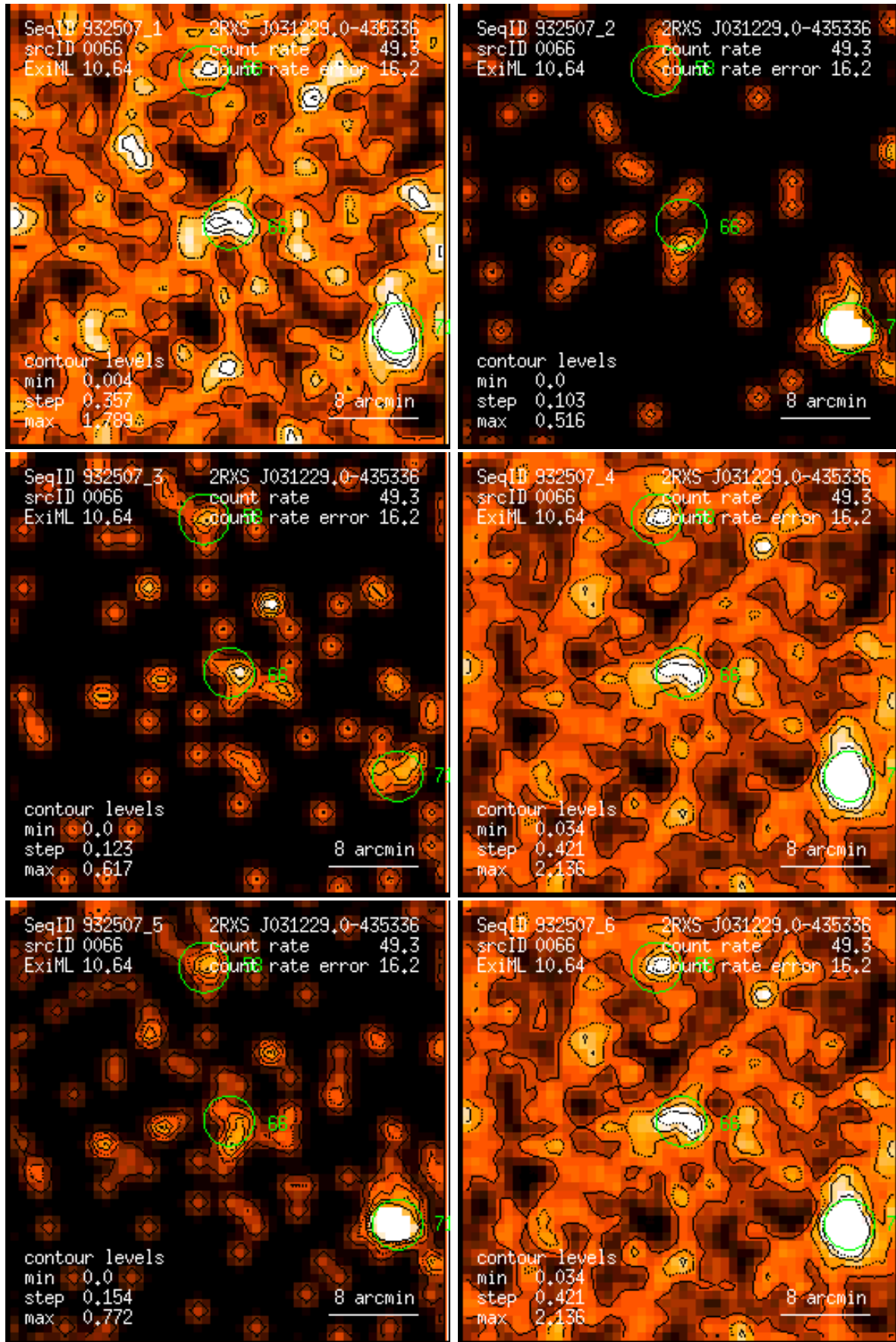
Figure 66: RASS 932507: detection 0066: band rate images, Gaussian filter: (1) PSPC channels 11 – 41, (2) 52 – 90, (3) 91 – 201, (4) 11 – 235, (5) 52 – 201, (6) 11 – 201. Broad band rates in counts/ks. Band rate contour levels in counts/ks/arcmin 2 .
