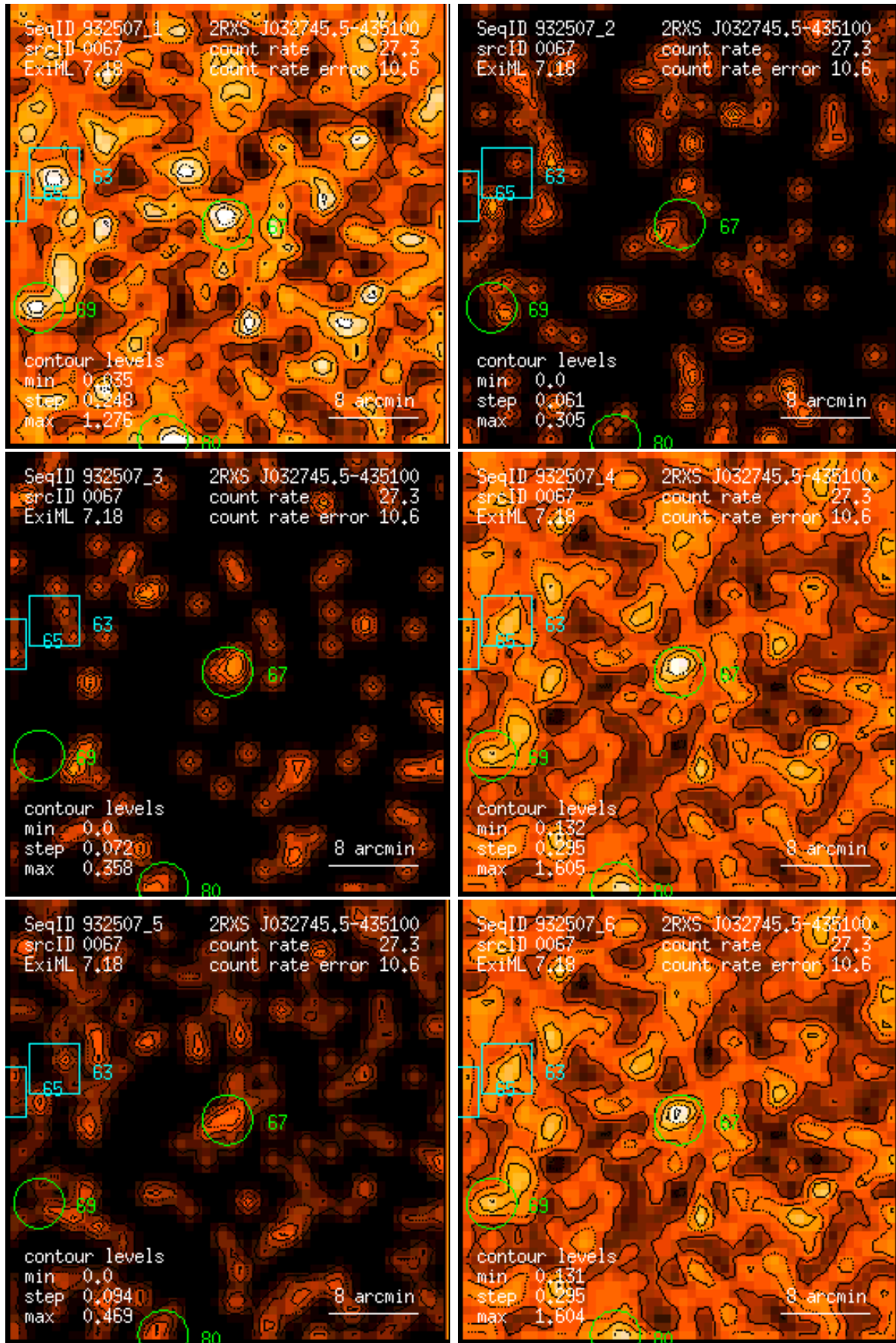
Figure 67: RASS 932507: detection 0067: band rate images, Gaussian filter: (1) PSPC channels 11 – 41, (2) 52 – 90, (3) 91 – 201, (4) 11 – 235, (5) 52 – 201, (6) 11 – 201. Broad band rates in counts/ks. Band rate contour levels in counts/ks/arcmin 2 .
