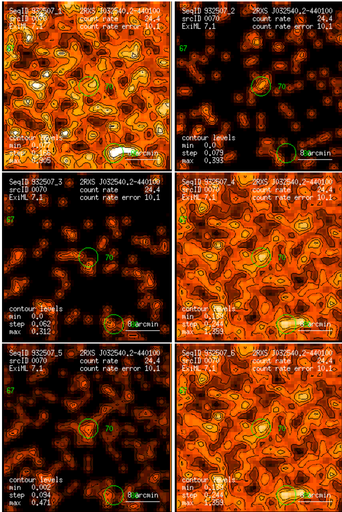
Figure 70: RASS 932507: detection 0070: band rate images, Gaussian filter: (1) PSPC channels 11 – 41, (2) 52 – 90, (3) 91 – 201, (4) 11 – 235, (5) 52 – 201, (6) 11 – 201. Broad band rates in counts/ks. Band rate contour levels in counts/ks/arcmin 2 .
