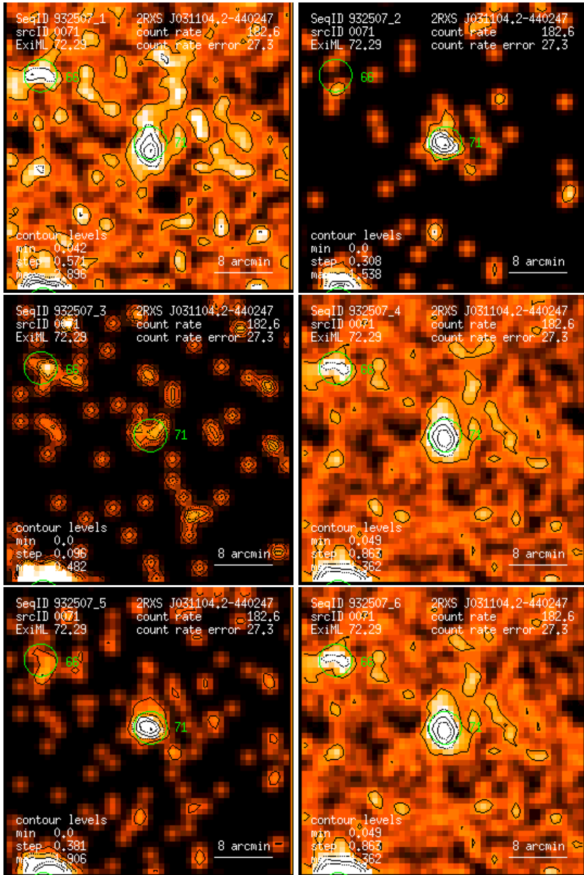
Figure 71: RASS 932507: detection 0071: band rate images, Gaussian filter: (1) PSPC channels 11 – 41, (2) 52 – 90, (3) 91 – 201, (4) 11 – 235, (5) 52 – 201, (6) 11 – 201. Broad band rates in counts/ks. Band rate contour levels in counts/ks/arcmin 2 .
