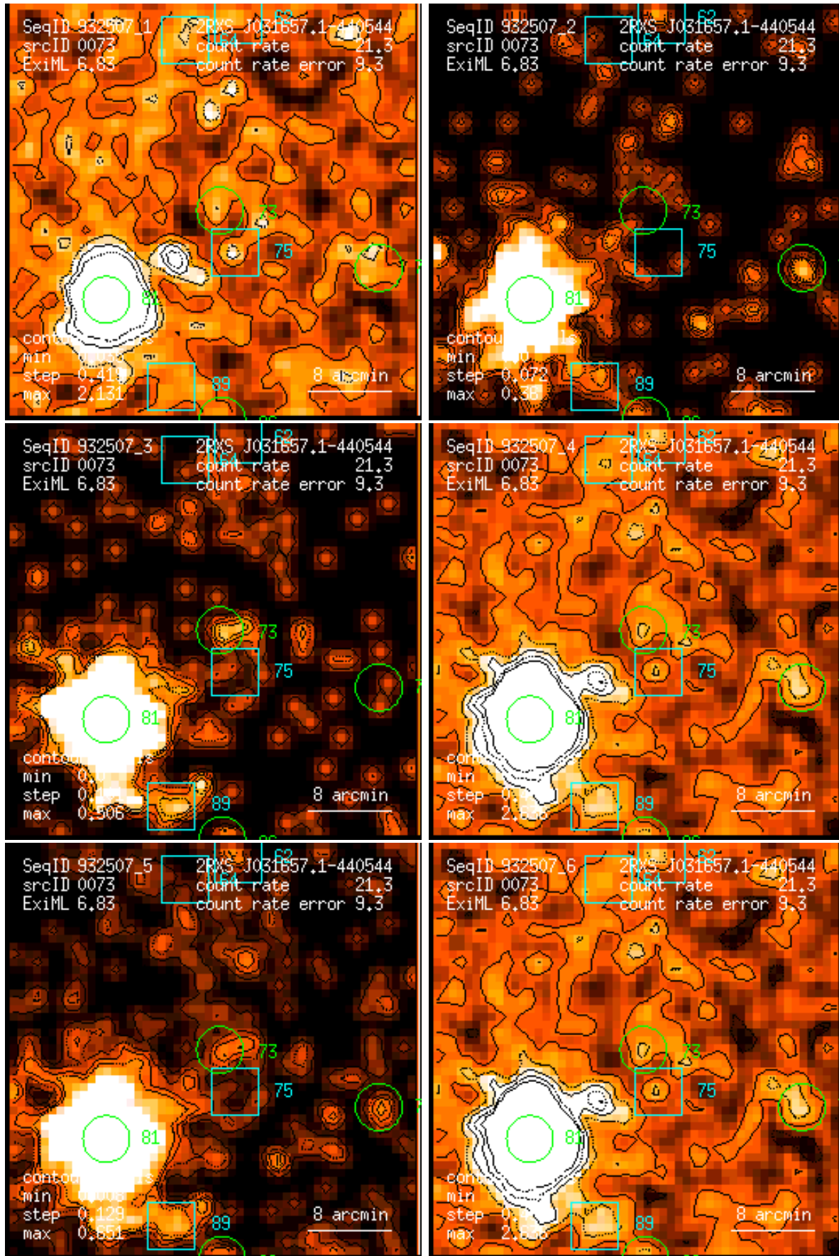
Figure 73: RASS 932507: detection 0073: band rate images, Gaussian filter: (1) PSPC channels 11 – 41, (2) 52 – 90, (3) 91 – 201, (4) 11 – 235, (5) 52 – 201, (6) 11 – 201. Broad band rates in counts/ks. Band rate contour levels in counts/ks/arcmin 2 .
