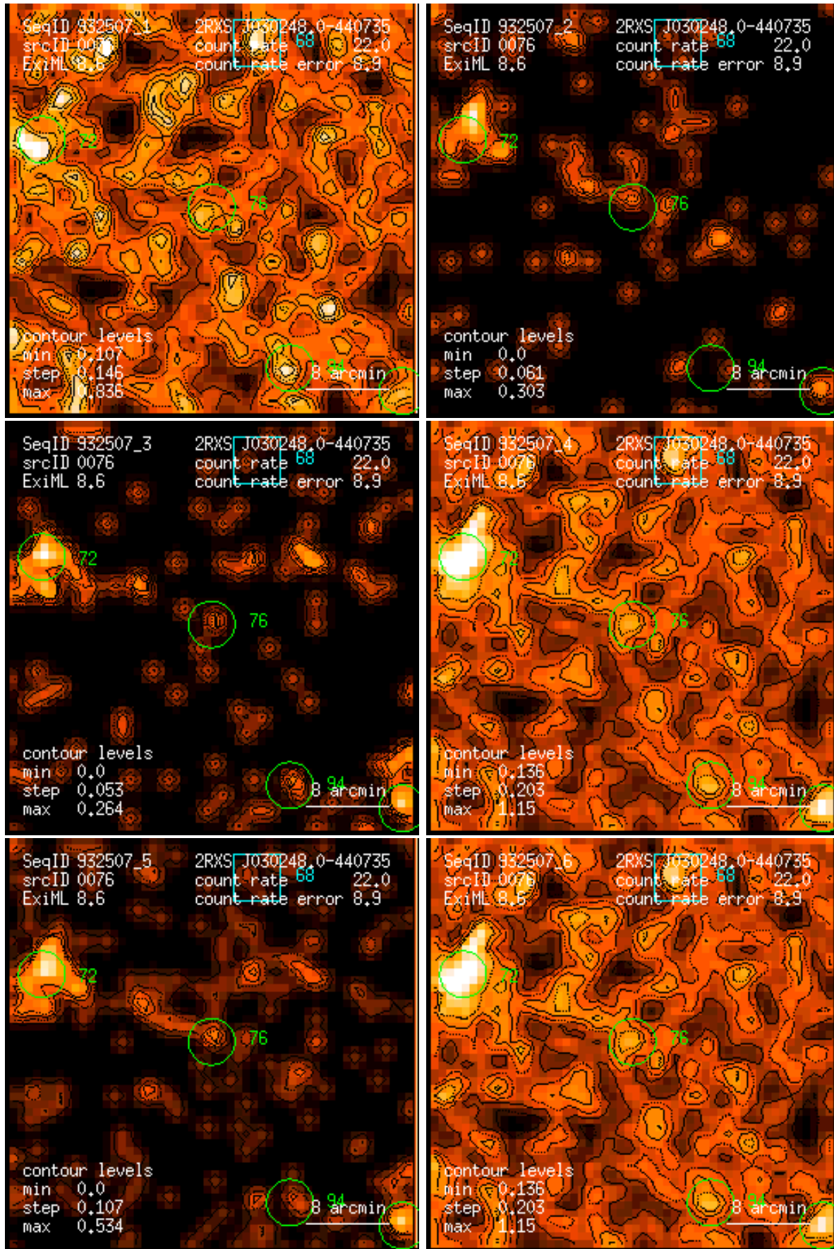
Figure 76: RASS 932507: detection 0076: band rate images, Gaussian filter: (1) PSPC channels 11 – 41, (2) 52 – 90, (3) 91 – 201, (4) 11 – 235, (5) 52 – 201, (6) 11 – 201. Broad band rates in counts/ks. Band rate contour levels in counts/ks/arcmin 2 .
