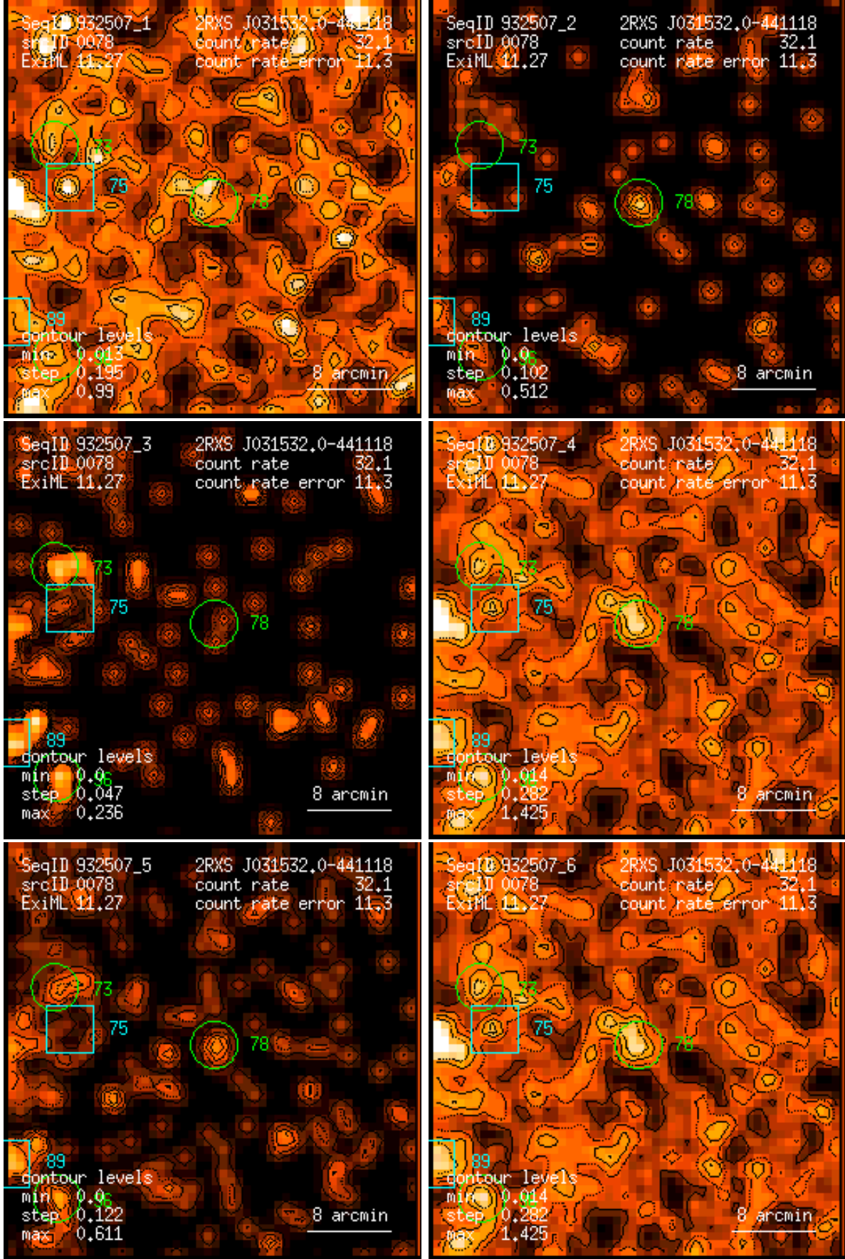
Figure 78: RASS 932507: detection 0078: band rate images, Gaussian filter: (1) PSPC channels 11 – 41, (2) 52 – 90, (3) 91 – 201, (4) 11 – 235, (5) 52 – 201, (6) 11 – 201. Broad band rates in counts/ks. Band rate contour levels in counts/ks/arcmin 2 .
