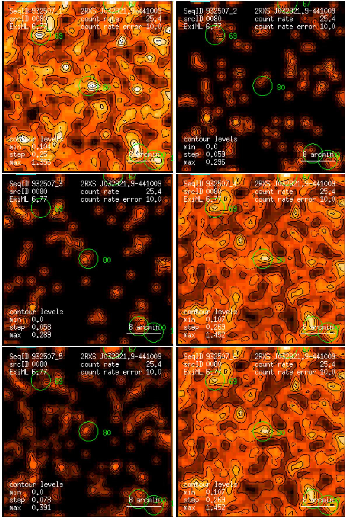
Figure 80: RASS 932507: detection 0080: band rate images, Gaussian filter: (1) PSPC channels 11 – 41, (2) 52 – 90, (3) 91 – 201, (4) 11 – 235, (5) 52 – 201, (6) 11 – 201. Broad band rates in counts/ks. Band rate contour levels in counts/ks/arcmin 2 .
