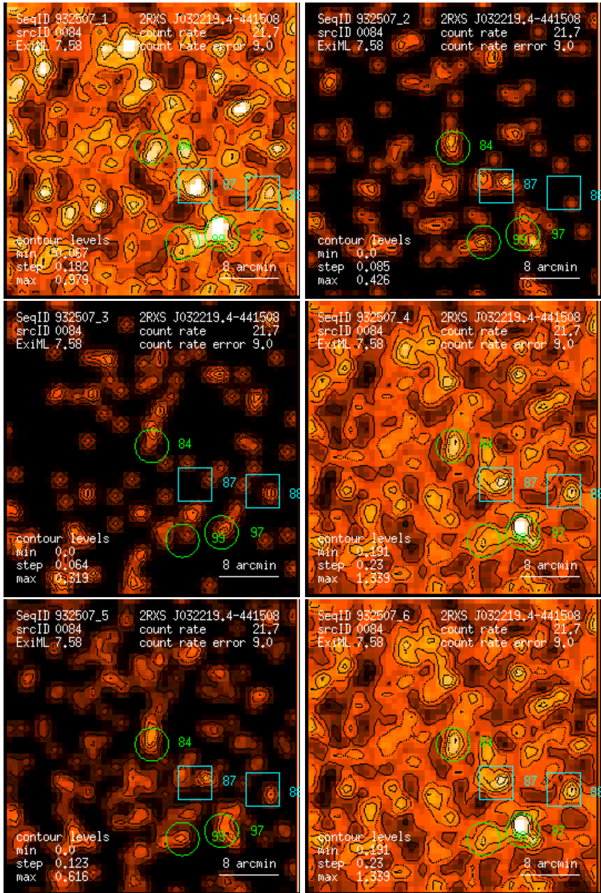
Figure 84: RASS 932507: detection 0084: band rate images, Gaussian filter: (1) PSPC channels 11 – 41, (2) 52 – 90, (3) 91 – 201, (4) 11 – 235, (5) 52 – 201, (6) 11 – 201. Broad band rates in counts/ks. Band rate contour levels in counts/ks/arcmin 2 .
