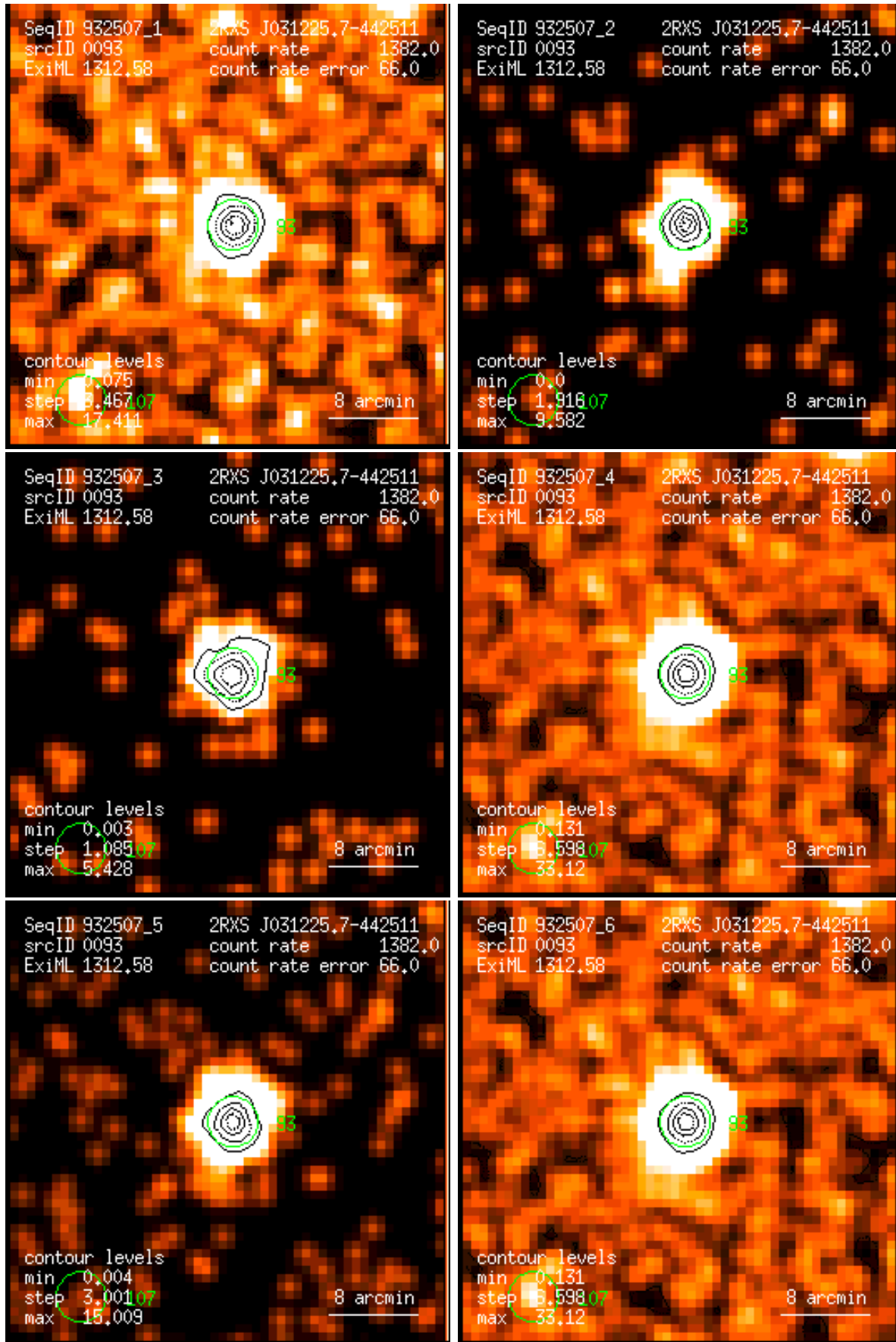
Figure 93: RASS 932507: detection 0093: band rate images, Gaussian filter: (1) PSPC channels 11 – 41, (2) 52 – 90, (3) 91 – 201, (4) 11 – 235, (5) 52 – 201, (6) 11 – 201. Broad band rates in counts/ks. Band rate contour levels in counts/ks/arcmin 2 .
