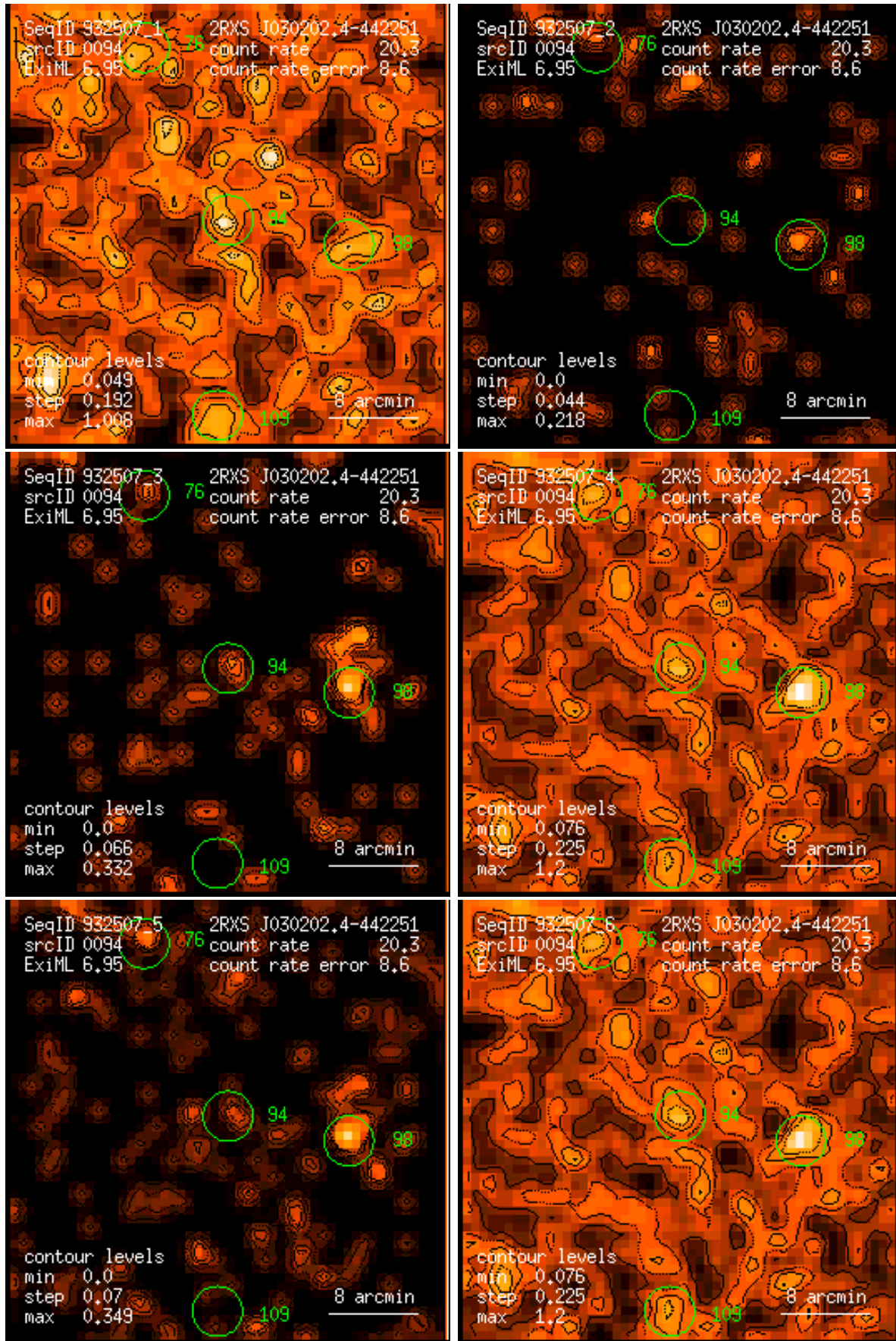
Figure 94: RASS 932507: detection 0094: band rate images, Gaussian filter: (1) PSPC channels 11 – 41, (2) 52 – 90, (3) 91 – 201, (4) 11 – 235, (5) 52 – 201, (6) 11 – 201. Broad band rates in counts/ks. Band rate contour levels in counts/ks/arcmin 2 .
