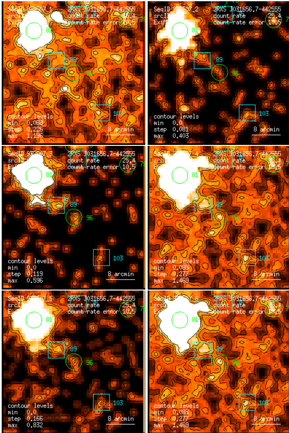
Figure 96: RASS 932507: detection 0096: band rate images, Gaussian filter: (1) PSPC channels 11 – 41, (2) 52 – 90, (3) 91 – 201, (4) 11 – 235, (5) 52 – 201, (6) 11 – 201. Broad band rates in counts/ks. Band rate contour levels in counts/ks/arcmin 2 .
