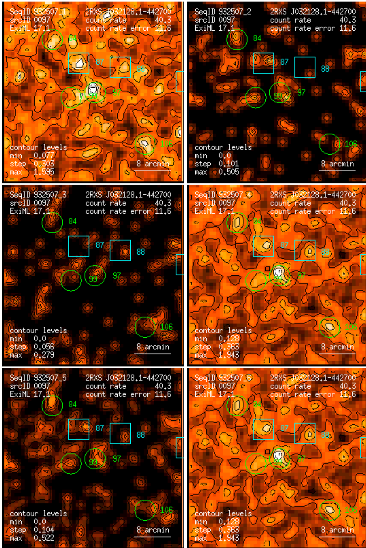
Figure 97: RASS 932507: detection 0097: band rate images, Gaussian filter: (1) PSPC channels 11 – 41, (2) 52 – 90, (3) 91 – 201, (4) 11 – 235, (5) 52 – 201, (6) 11 – 201. Broad band rates in counts/ks. Band rate contour levels in counts/ks/arcmin 2 .
