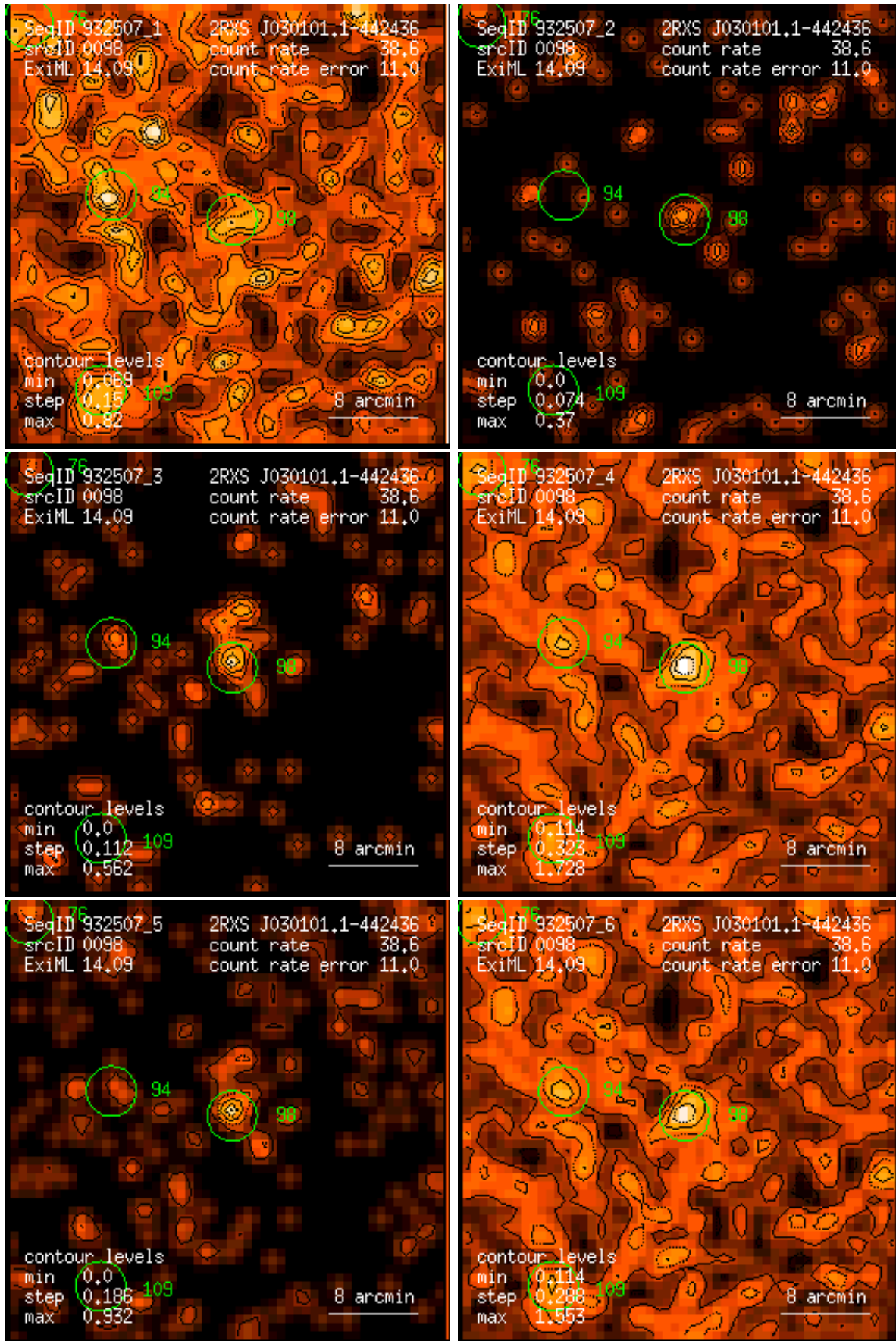
Figure 98: RASS 932507: detection 0098: band rate images, Gaussian filter: (1) PSPC channels 11 – 41, (2) 52 – 90, (3) 91 – 201, (4) 11 – 235, (5) 52 – 201, (6) 11 – 201. Broad band rates in counts/ks. Band rate contour levels in counts/ks/arcmin 2 .
