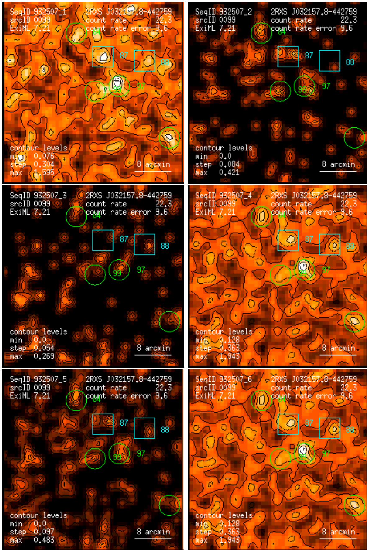
Figure 99: RASS 932507: detection 0099: band rate images, Gaussian filter: (1) PSPC channels 11 – 41, (2) 52 – 90, (3) 91 – 201, (4) 11 – 235, (5) 52 – 201, (6) 11 – 201. Broad band rates in counts/ks. Band rate contour levels in counts/ks/arcmin 2 .
