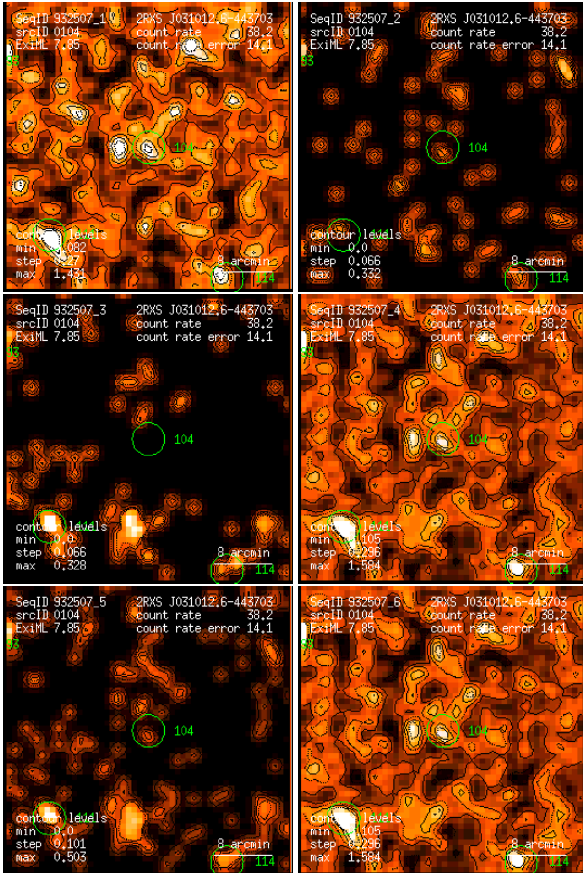
Figure 104: RASS 932507: detection 0104: band rate images, Gaussian filter: (1) PSPC channels 11 – 41, (2) 52 – 90, (3) 91 – 201, (4) 11 – 235, (5) 52 – 201, (6) 11 – 201. Broad band rates in counts/ks. Band rate contour levels in counts/ks/arcmin 2 .
