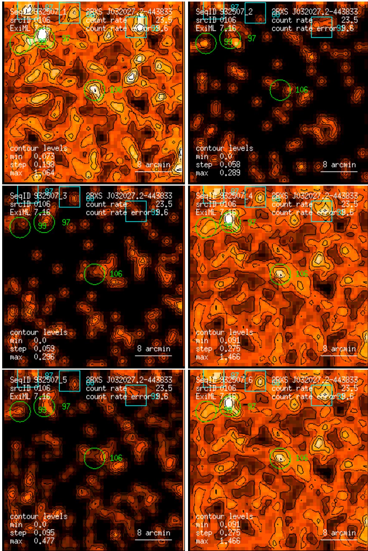
Figure 106: RASS 932507: detection 0106: band rate images, Gaussian filter: (1) PSPC channels 11 – 41, (2) 52 – 90, (3) 91 – 201, (4) 11 – 235, (5) 52 – 201, (6) 11 – 201. Broad band rates in counts/ks. Band rate contour levels in counts/ks/arcmin 2 .
