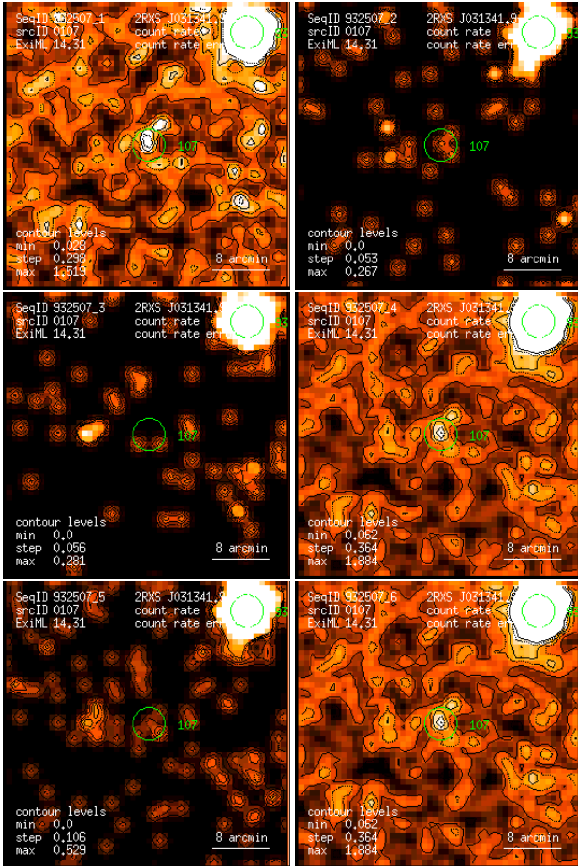
Figure 107: RASS 932507: detection 0107: band rate images, Gaussian filter: (1) PSPC channels 11 – 41, (2) 52 – 90, (3) 91 – 201, (4) 11 – 235, (5) 52 – 201, (6) 11 – 201. Broad band rates in counts/ks. Band rate contour levels in counts/ks/arcmin 2 .
