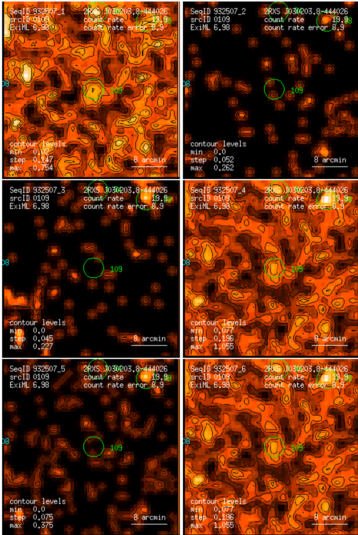
Figure 109: RASS 932507: detection 0109: band rate images, Gaussian filter: (1) PSPC channels 11 – 41, (2) 52 – 90, (3) 91 – 201, (4) 11 – 235, (5) 52 – 201, (6) 11 – 201. Broad band rates in counts/ks. Band rate contour levels in counts/ks/arcmin 2 .
