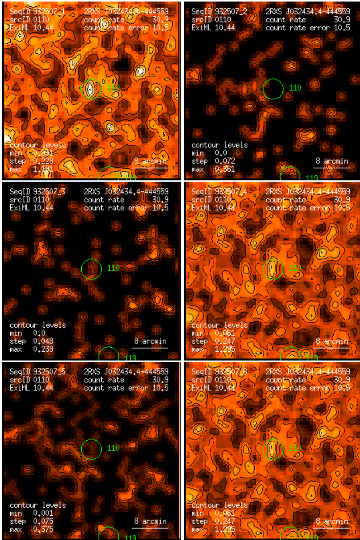
Figure 110: RASS 932507: detection 0110: band rate images, Gaussian filter: (1) PSPC channels 11 – 41, (2) 52 – 90, (3) 91 – 201, (4) 11 – 235, (5) 52 – 201, (6) 11 – 201. Broad band rates in counts/ks. Band rate contour levels in counts/ks/arcmin 2 .
