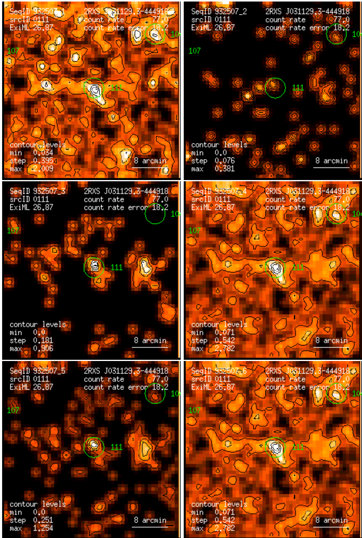
Figure 111: RASS 932507: detection 0111: band rate images, Gaussian filter: (1) PSPC channels 11 – 41, (2) 52 – 90, (3) 91 – 201, (4) 11 – 235, (5) 52 – 201, (6) 11 – 201. Broad band rates in counts/ks. Band rate contour levels in counts/ks/arcmin 2 .
