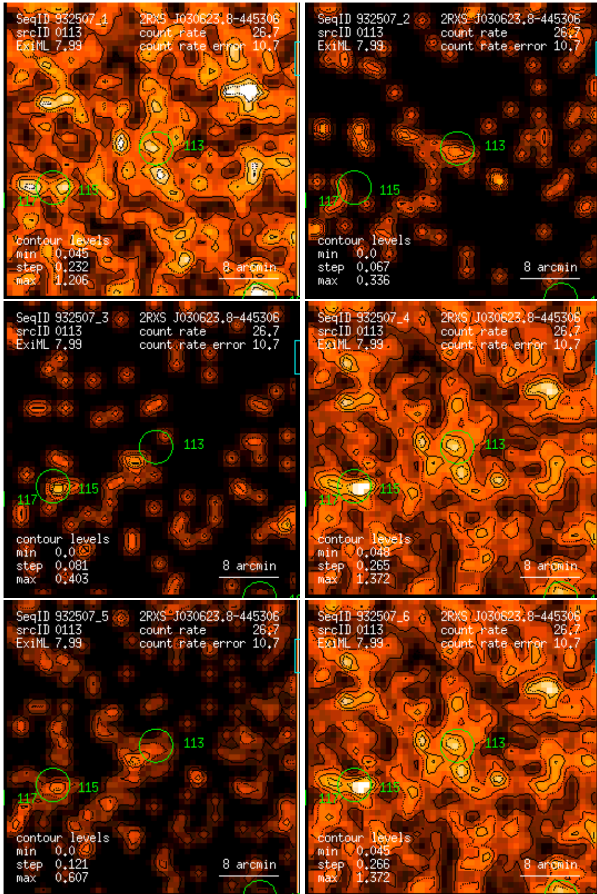
Figure 113: RASS 932507: detection 0113: band rate images, Gaussian filter: (1) PSPC channels 11 – 41, (2) 52 – 90, (3) 91 – 201, (4) 11 – 235, (5) 52 – 201, (6) 11 – 201. Broad band rates in counts/ks. Band rate contour levels in counts/ks/arcmin 2 .
