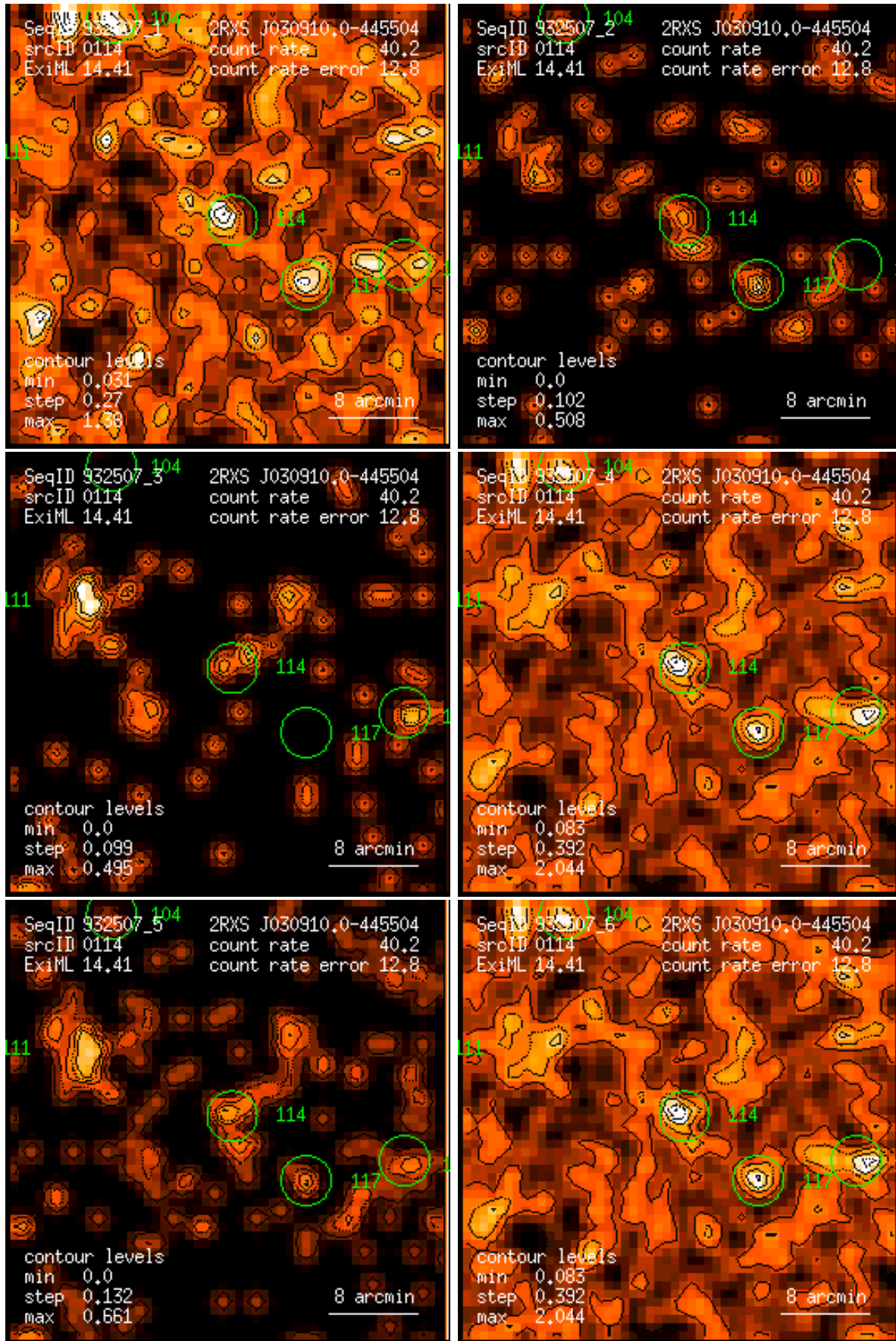
Figure 114: RASS 932507: detection 0114: band rate images, Gaussian filter: (1) PSPC channels 11 – 41, (2) 52 – 90, (3) 91 – 201, (4) 11 – 235, (5) 52 – 201, (6) 11 – 201. Broad band rates in counts/ks. Band rate contour levels in counts/ks/arcmin 2 .
