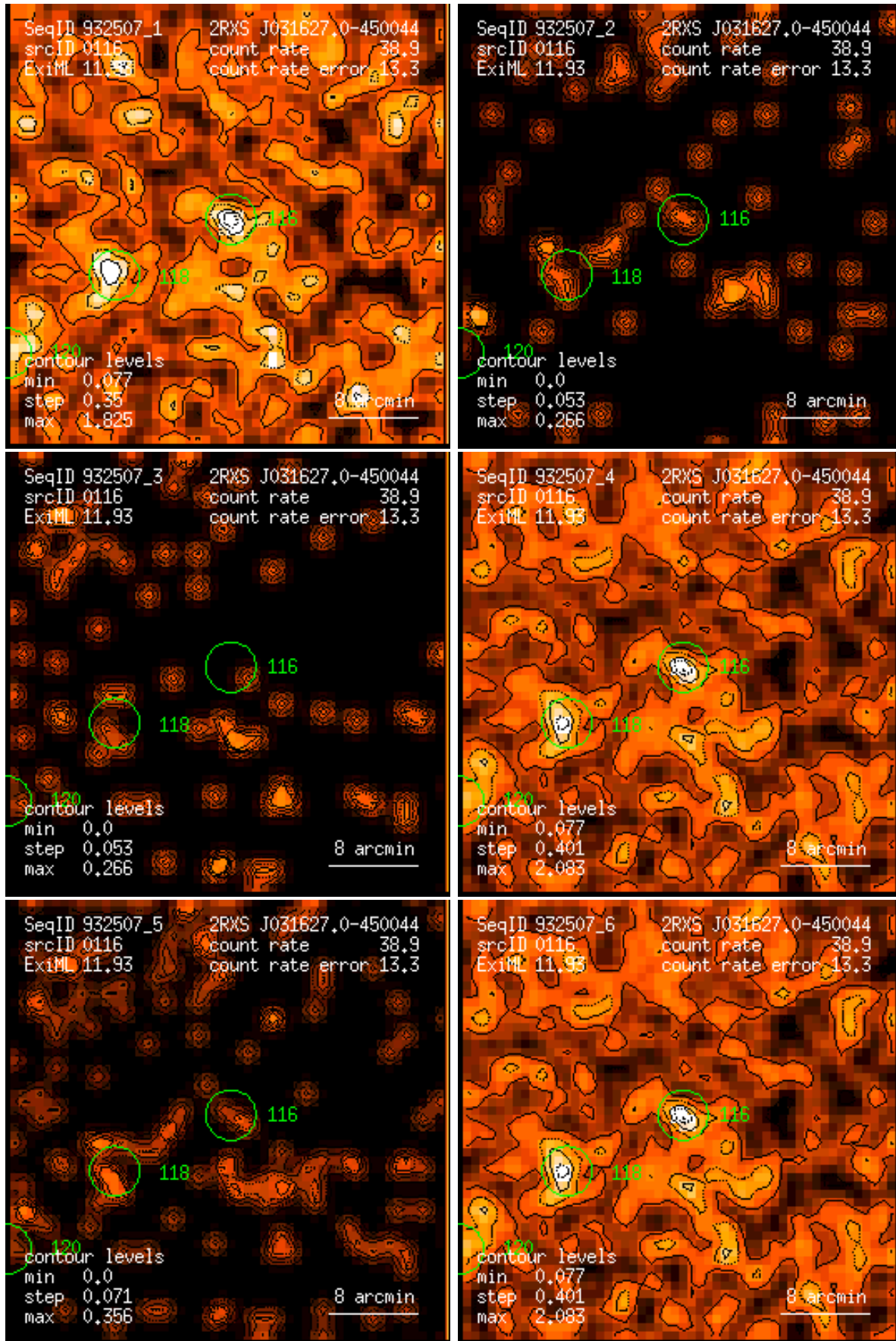
Figure 116: RASS 932507: detection 0116: band rate images, Gaussian filter: (1) PSPC channels 11 – 41, (2) 52 – 90, (3) 91 – 201, (4) 11 – 235, (5) 52 – 201, (6) 11 – 201. Broad band rates in counts/ks. Band rate contour levels in counts/ks/arcmin 2 .
