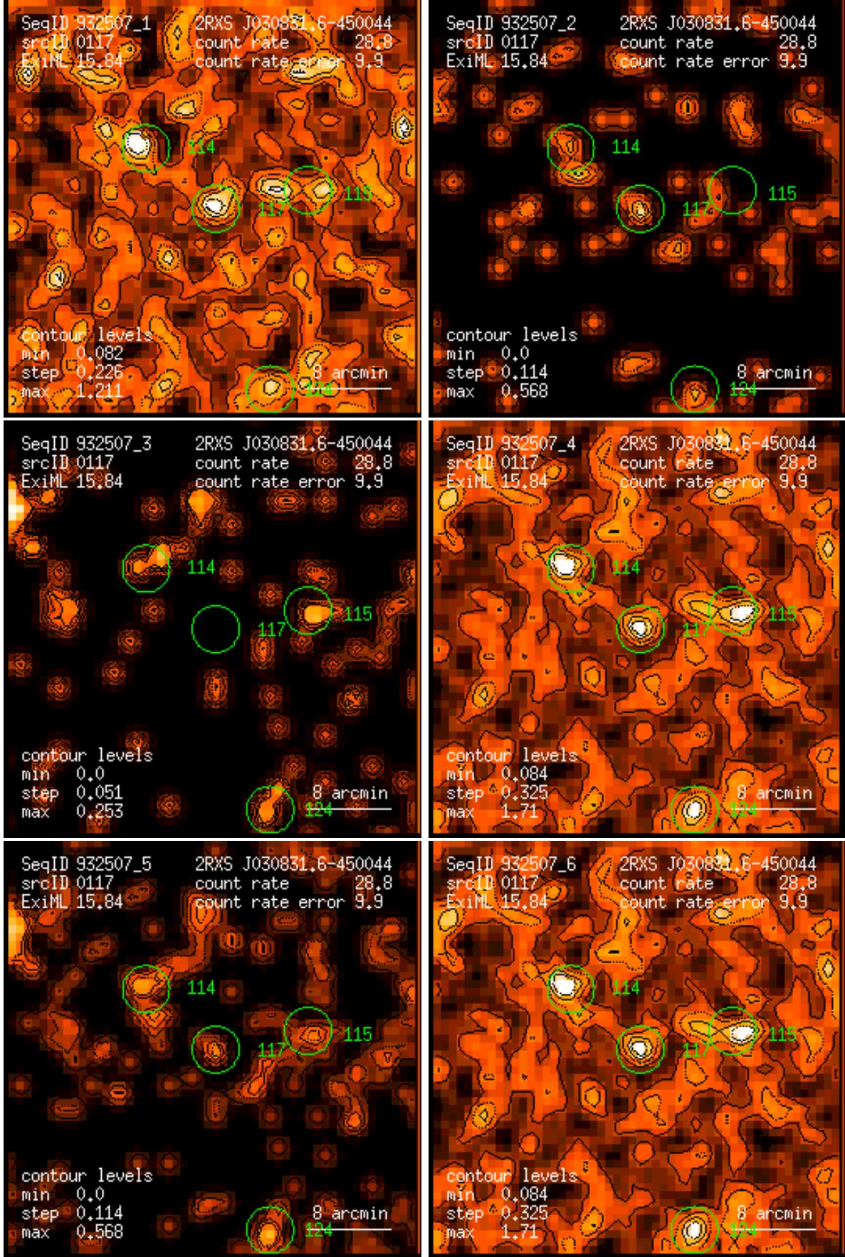
Figure 117: RASS 932507: detection 0117: band rate images, Gaussian filter: (1) PSPC channels 11 – 41, (2) 52 – 90, (3) 91 – 201, (4) 11 – 235, (5) 52 – 201, (6) 11 – 201. Broad band rates in counts/ks. Band rate contour levels in counts/ks/arcmin 2 .
